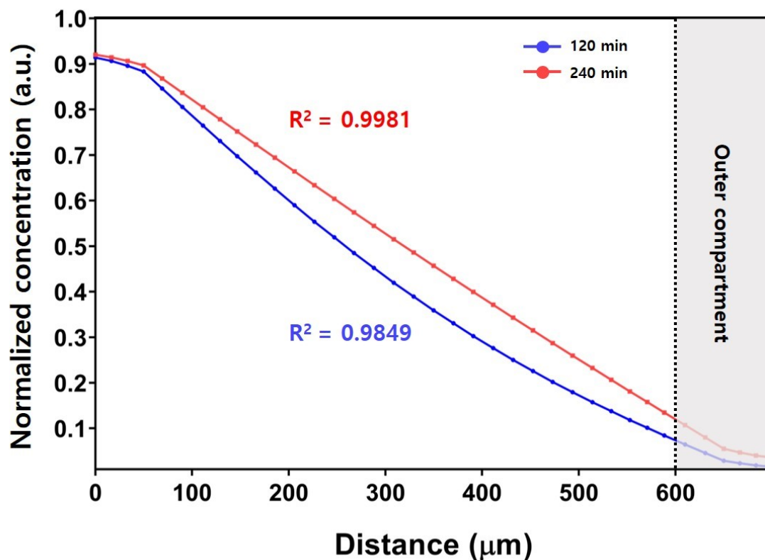
Figure S1. The diffusion profile of the chemo-attractants was characterized by measuring the gradient and normalized concentration plot over a period of 120 and 240 min (Linearity R^2 values are 0.9849 and 0.9981, respectively) using COMSOL software.
