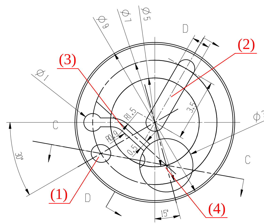
Bottom view
