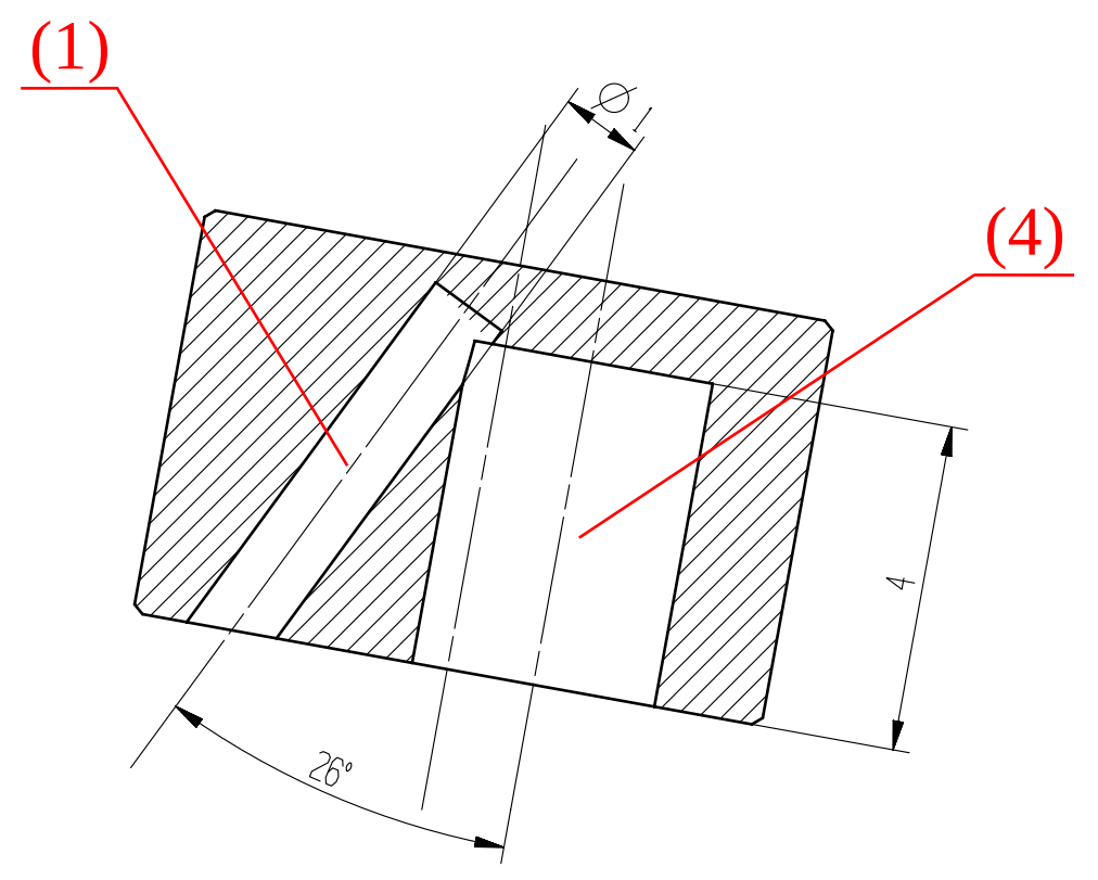
Section C-C
