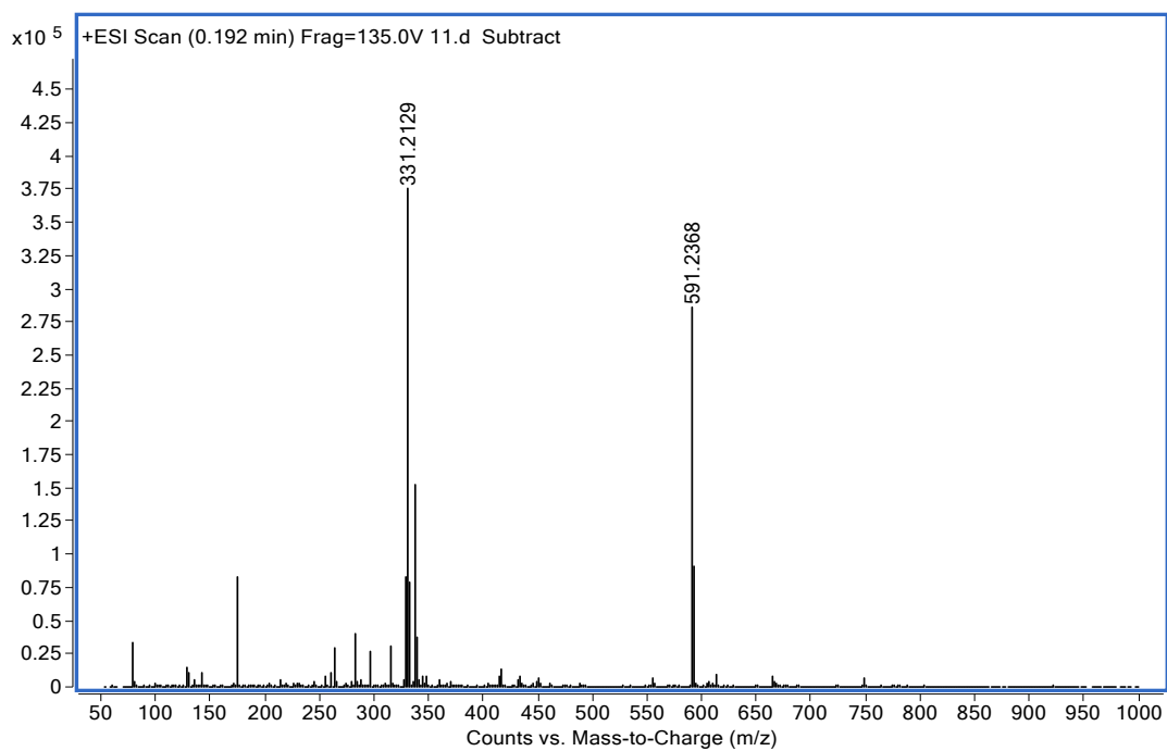
HRMS spectrum of Compound 8.
