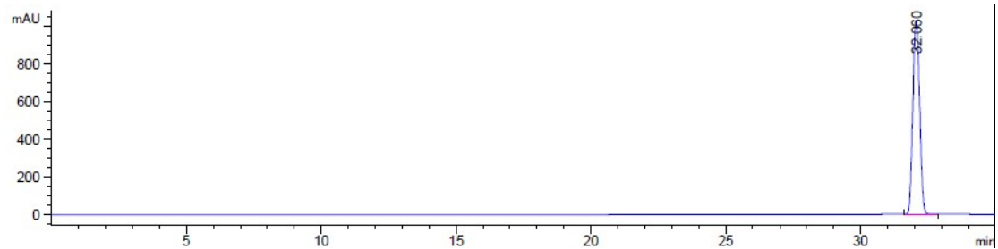
HPLC spectrum of Compound 4.
