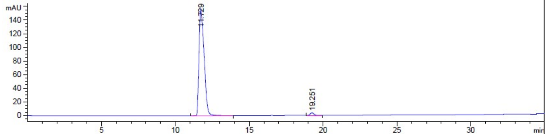
HPLC spectrum of Compound 2.
