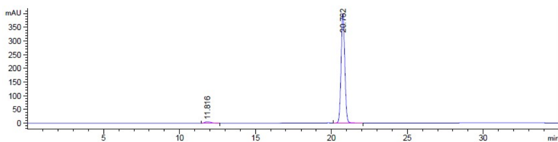
HPLC spectrum of Compound 6.
