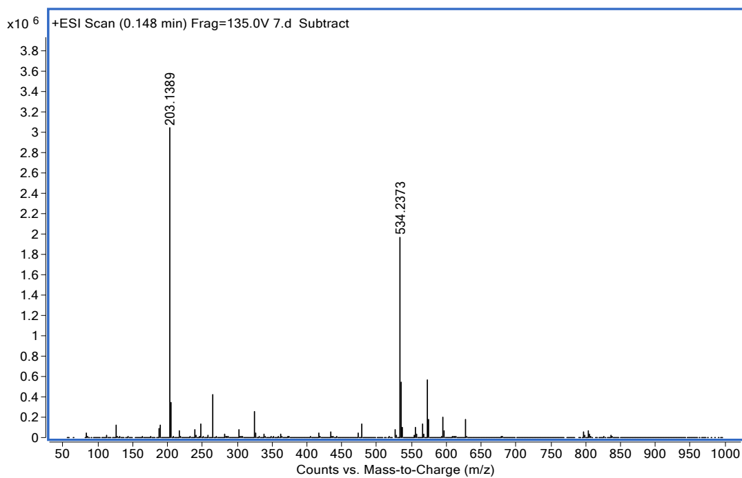
HRMS spectrum of Compound 6.
