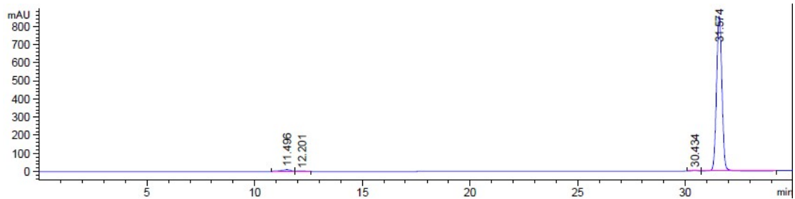
HPLC spectrum of Compound 5.
