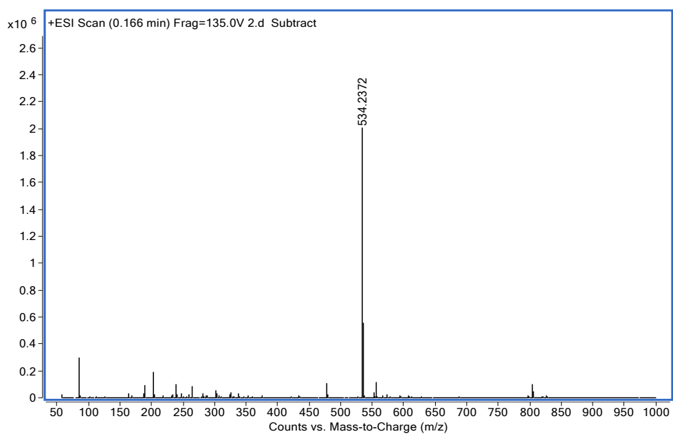
HRMS spectrum of Compound 1.
