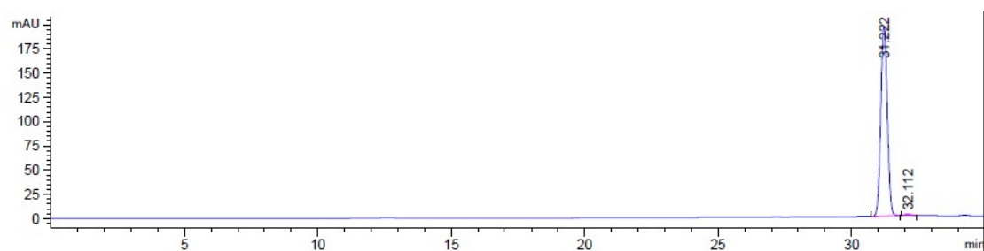
HPLC spectrum of Compound 10.
