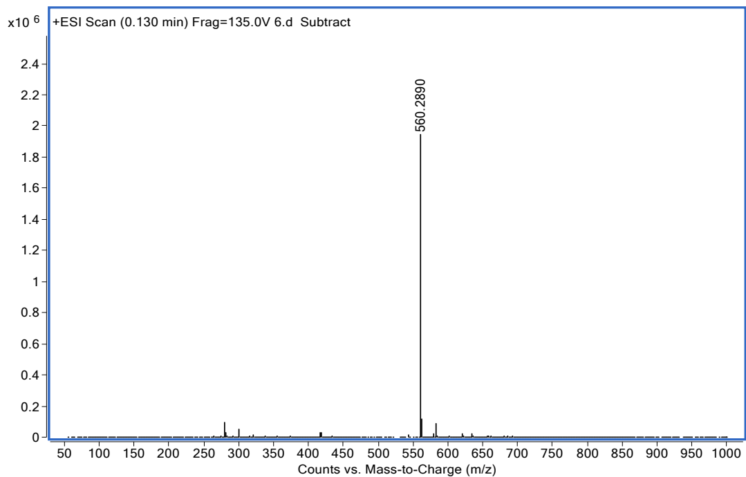
HRMS spectrum of Compound 5.
