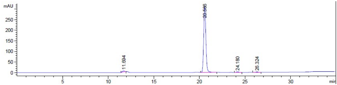
HPLC spectrum of Compound 3.
