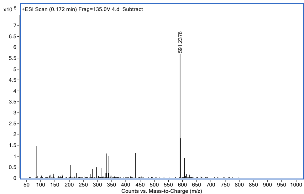
HRMS spectrum of Compound 3.
