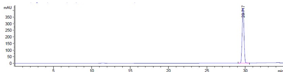
HPLC spectrum of Compound 9.
