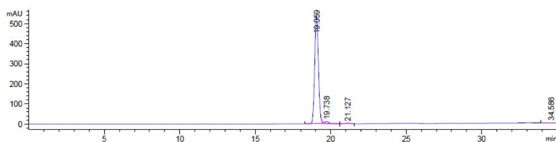
HPLC spectrum of Compound 8.
