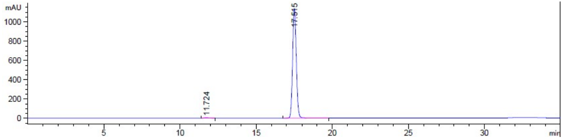
HPLC spectrum of Compound 1.
