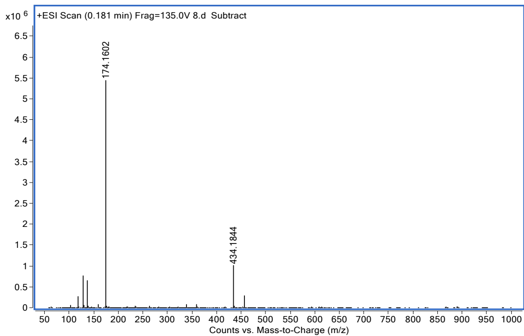
HRMS spectrum of Compound 7.
