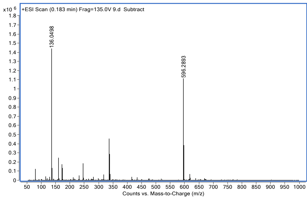
HRMS spectrum of Compound 9.
