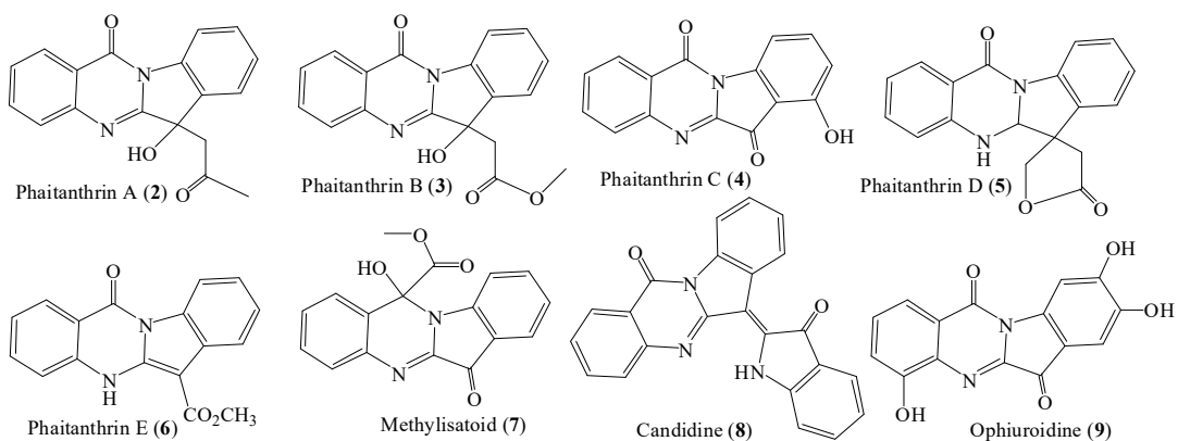
Scheme S1 Tryptanthrin derivatives isolated from natural sources
