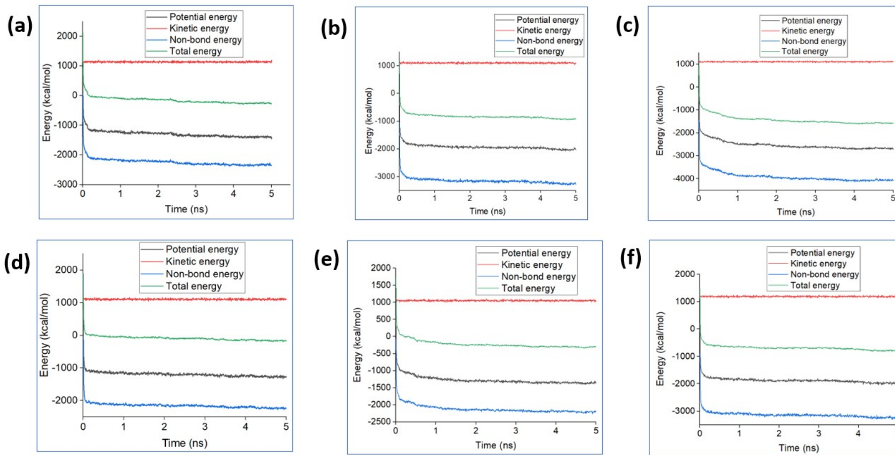
Figure S7: Thermodynamic equilibrium energies observed during 5.0 ns simulation time for the systems (a) Cort-4VP, (b) Cort-AA, (c) Cort-AM, (d) Cort-GMA, (e) Cort-HEMA and (f) Cort-MAA
