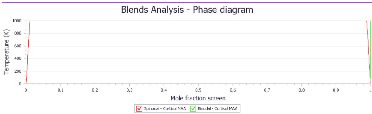
Figure S5: Cort-HEMA phase diagram
