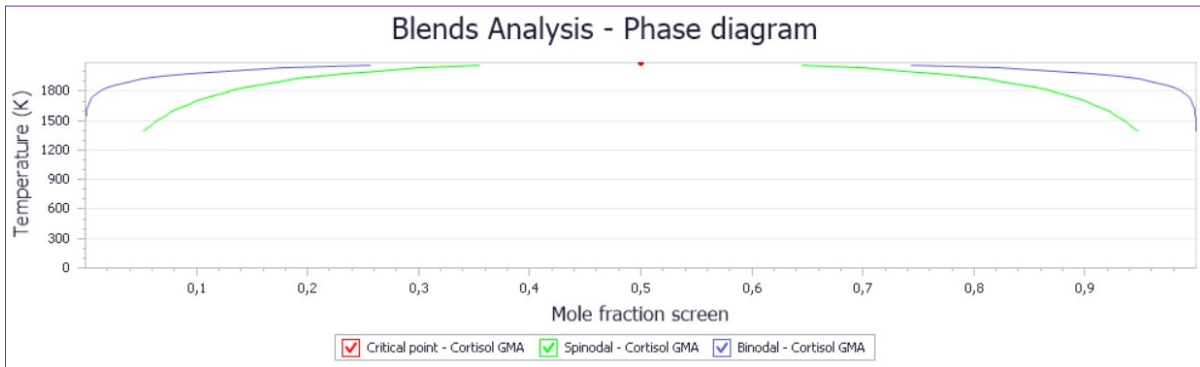
Figure S4: Cort-GMA phase diagram
