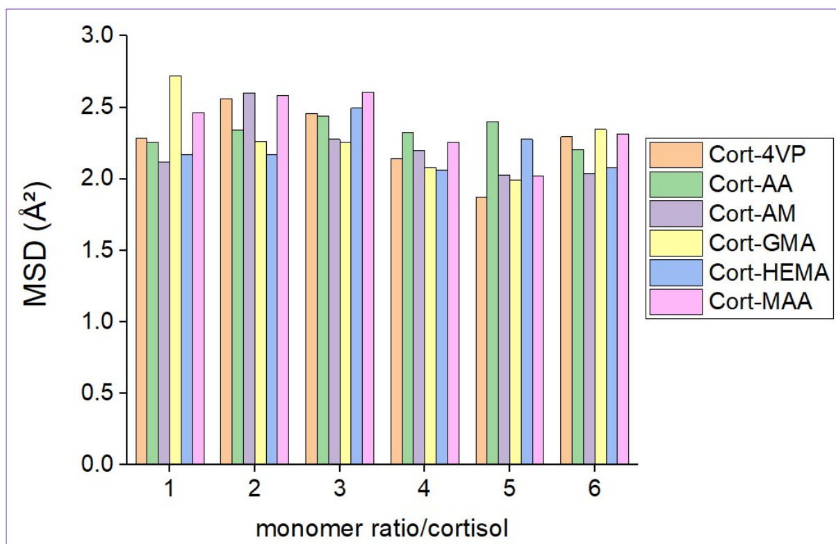
Figure S8: The mean square displacement (MSD) maximal for all the ratios
