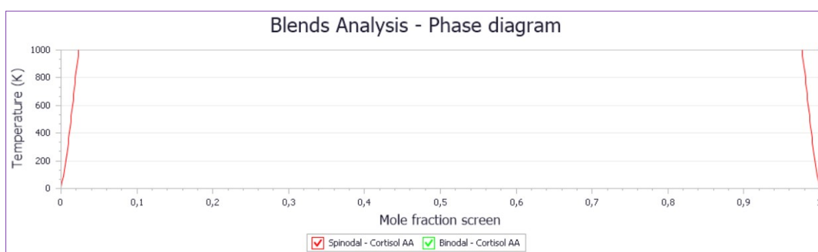
Figure S2: Cort-AA phase diagram
