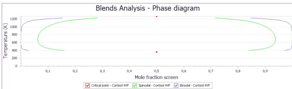
Figure S1: Cort-4VP phase diagram
