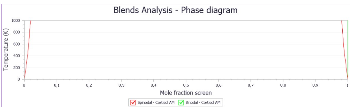
Figure S3: Cort-AM phase diagram
