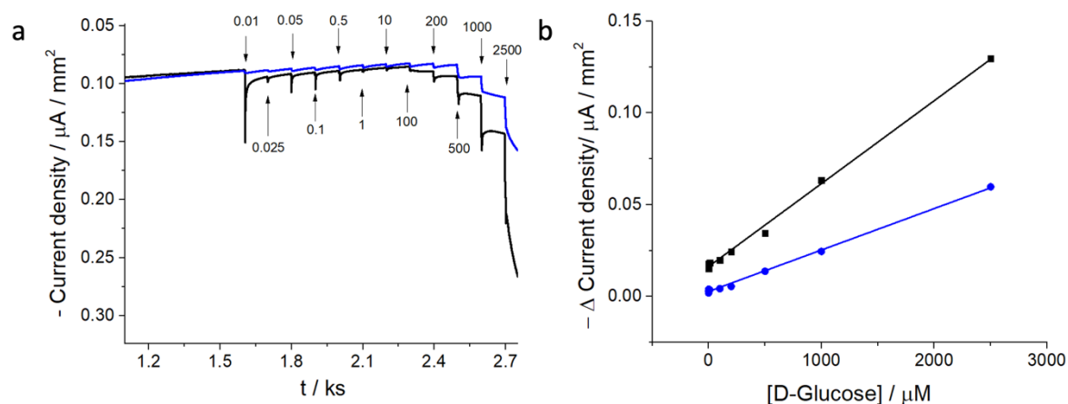
Figure S7. Evaluation of the stability of the sensor. (a) Chronoamperometric measurements of standard additions for freshly prepared (black) and stressed IO-based biosensor stored in PBS and tested after 72 h (blue). The curves are registered in PBS solution at RT, E = + 0.65 V vs Ag/AgCl (3 M KCl). The additions indicated by the arrows are expressed in \mu\text{M} . (b) Change in current density at t=0 (black) and at t=72\text{h} (blue) upon standard additions of glucose. The slopes are respectively 4.52 \cdot 10^{-5} \mu\text{A} / \mu\text{M} for the biosensor at first use and 2.26 \cdot 10^{-5} \mu\text{A} / \mu\text{M} for the biosensor after 72h. 50% of the activity is retained after 72h.
