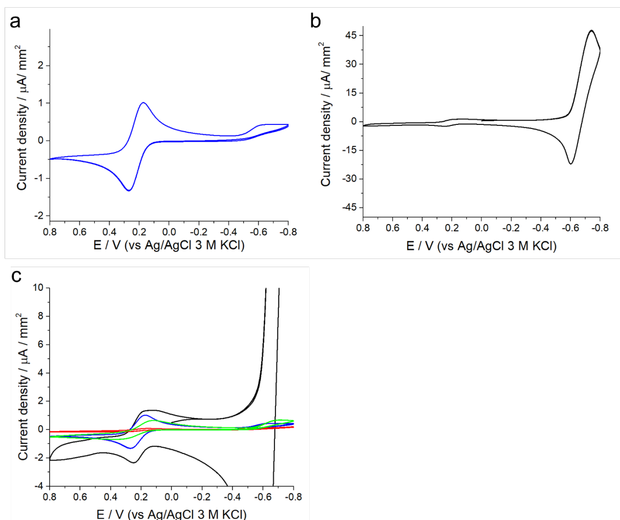
Figure S3. Cyclic voltammograms of ITO-coated glass slide (a), Pt (b), and overlay of the voltammograms of the isolated components and final electrode (c- ITO-coated glass slide (blue), Pt (black), ITO glass slide covered with AZO (red) and IO covered with AZO (green)). The CVs are registered in a solution of 2 mM FcMeOH in PB. Potential scan from -0.8 to 0.8 V vs. Ag/AgCl (3 M KCl), scan rate 20 mV/s.
