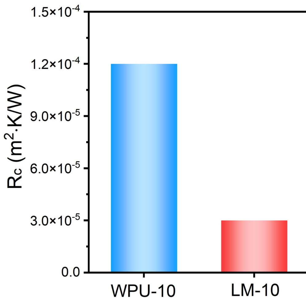
Fig. S12. R_s - R_c of the LM-10 bulk and the WPU-10 composite.
