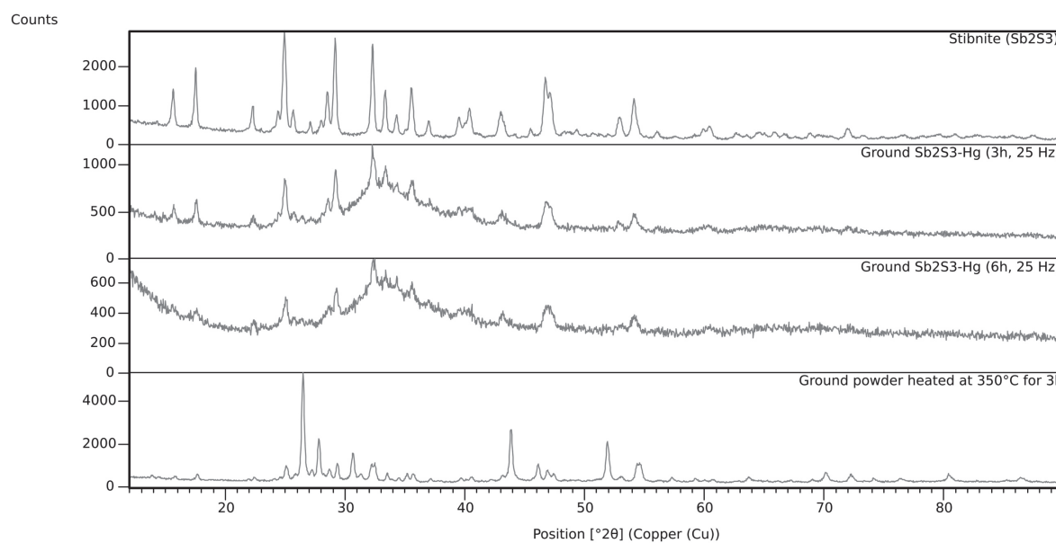
Figure S21. Comparison between XRPD pattern of reagent stibnite Sb 2 S 3 (up), of the ground powder obtained from Hg and Sb 2 S 3 (middle) and of the ground powder heating at 350°C (bottom). Phase identification was performed using the PDF 2 Release 2004 database.
