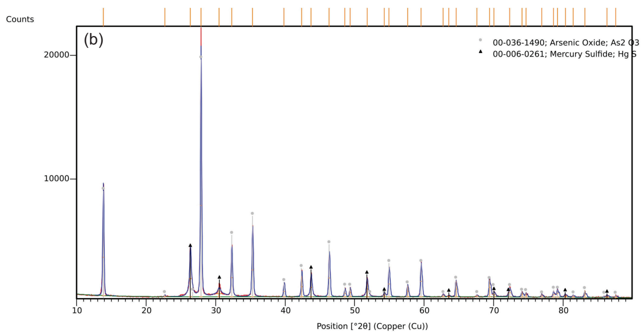
Figure S13. XRPD pattern of the residual powder (a. bottom of the flask; b. scratched from the glassware) obtained upon grinding \text{As}_2\text{S}_3 with Hg (three hours at 25Hz) and heating the so-obtained powder at 350^{\circ}\text{C} . Phase identification was performed using the PDF 2 Release 2004 database.
