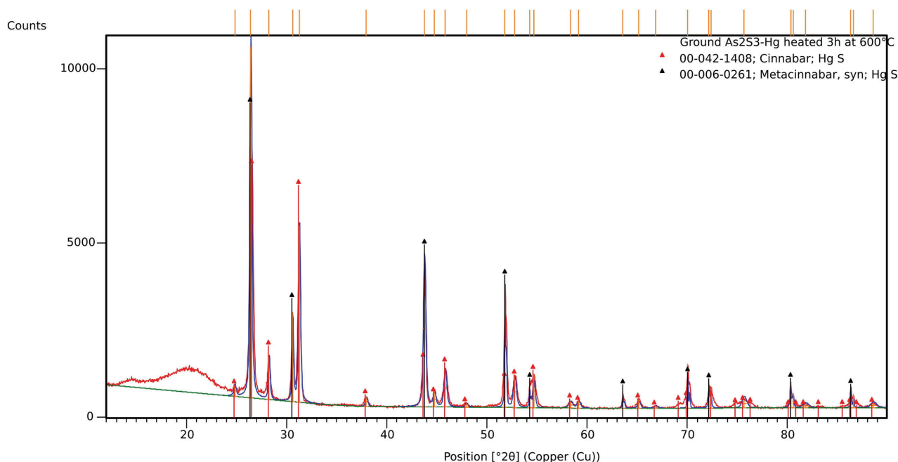
Figure S14. XRPD pattern of the residual powder obtained upon grinding \text{As}_2\text{S}_3 with Hg (three hours at 25Hz) and heating the so-obtained powder at 600°C. Phase identification was performed using the PDF 2 Release 2004 database.
