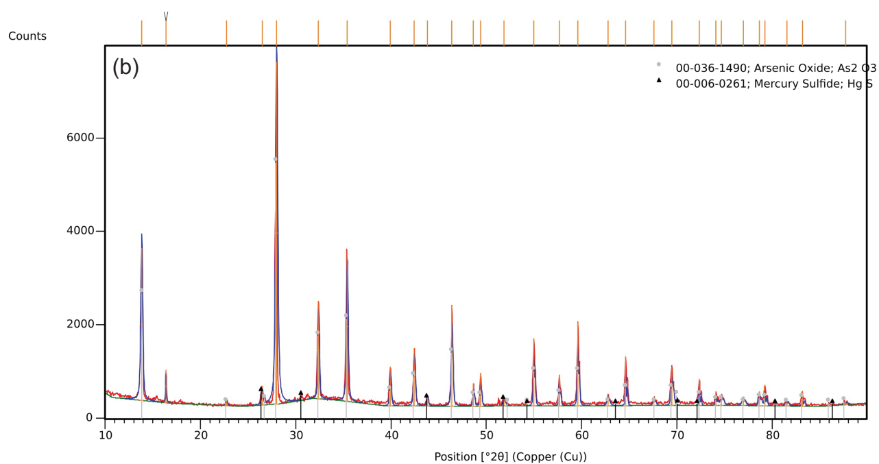
Figure S18. XRPD pattern of the residual powder (a. bottom of the flask; b. scratched from the upper part of the Kjeldahl flask) obtained upon grinding As 4 S 4 with Hg (three hours at 25Hz) and heating the so-obtained powder at 350°C. Phase identification was performed using the PDF 2 Release 2004 database.
