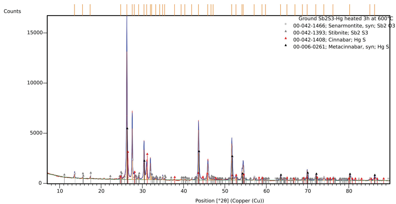
Figure S25. XRPD pattern of the residual powder obtained upon grinding Sb 2 S 3 with Hg (three hours at 25Hz) and heating the so-obtained powder at 600°C. Phase identification was performed using the PDF 2 Release 2004 database.
