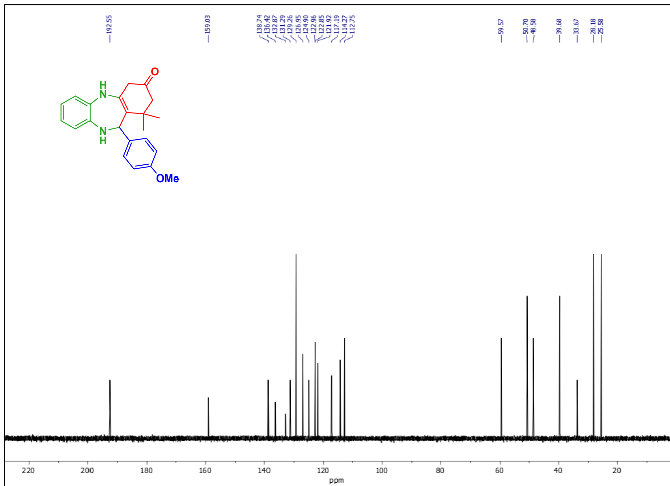
^{13}\text{C} -NMR spectra of 4h
