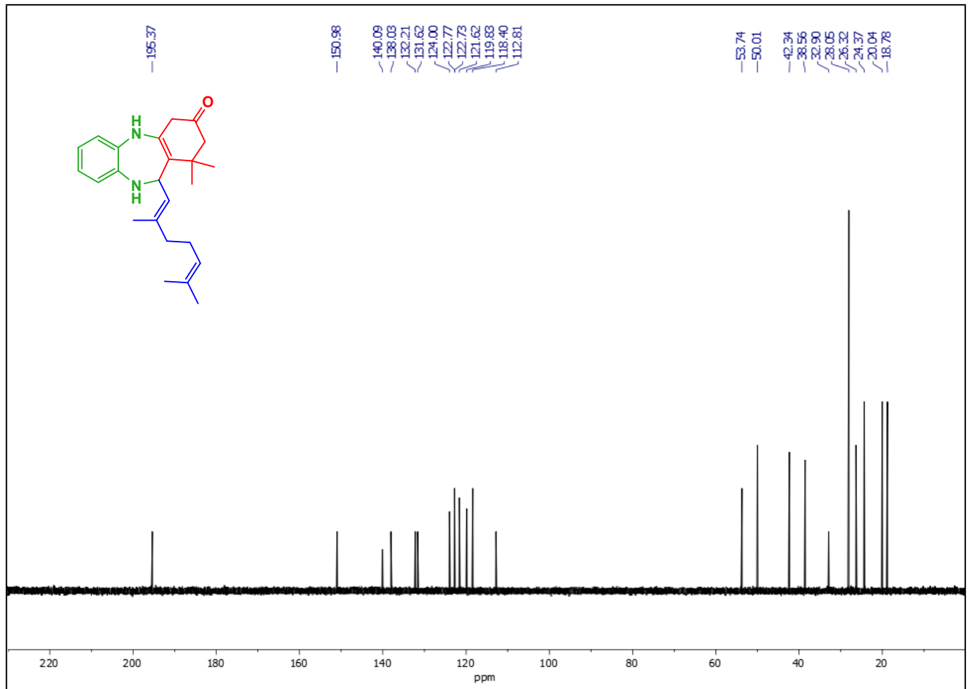
13 C-NMR spectra of 4m
