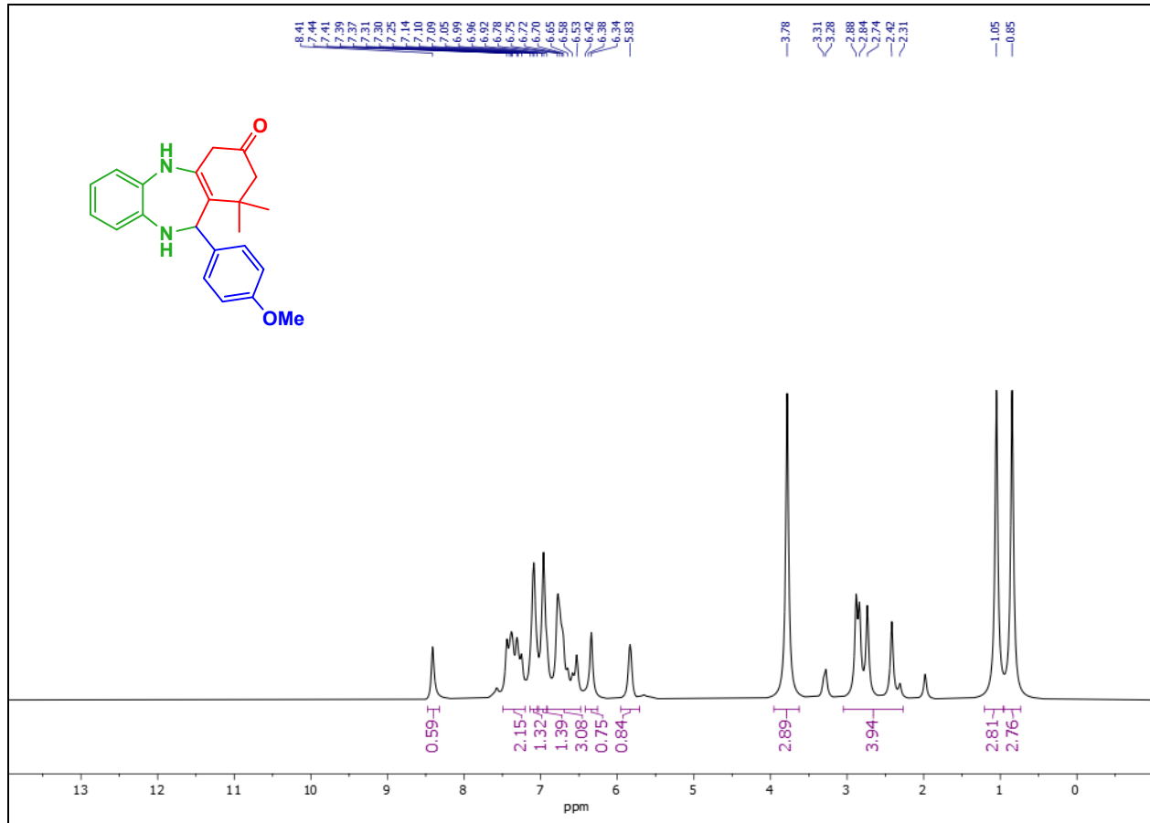
1 H-NMR spectra of 4h
