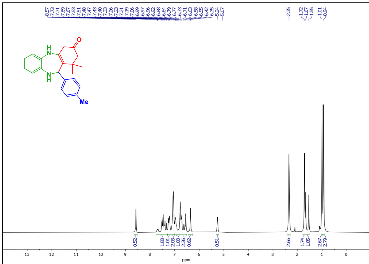
1 H-NMR spectra of 4k
