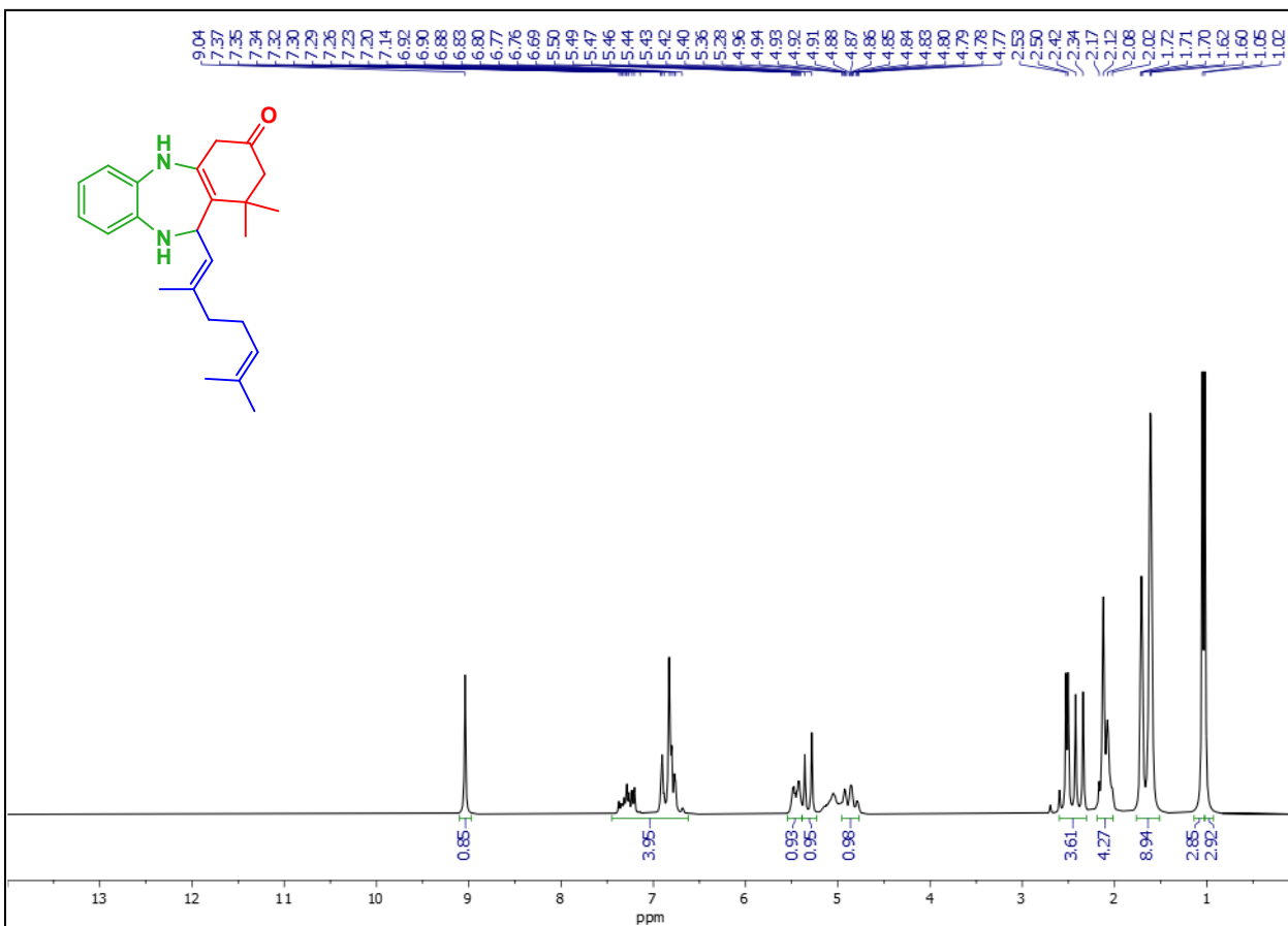
1 H-NMR spectra of 4m
