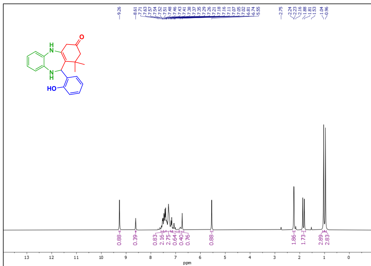
1 H-NMR spectra of 4b
