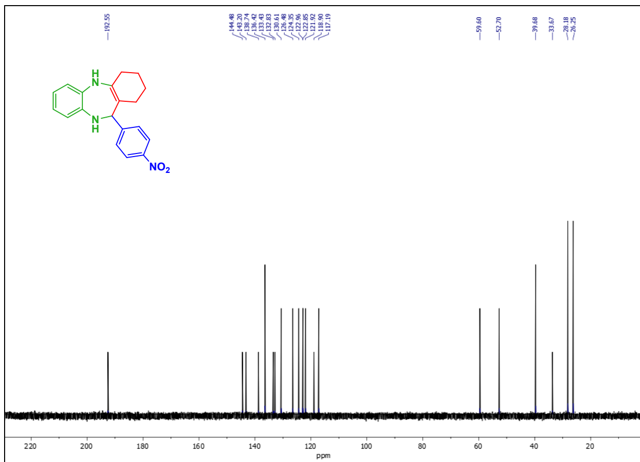
13 C-NMR spectra of 4c
