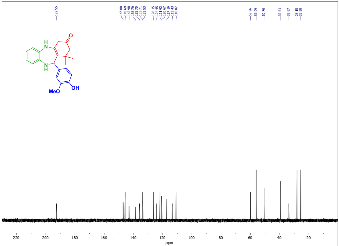
13 C-NMR spectra of 4i
