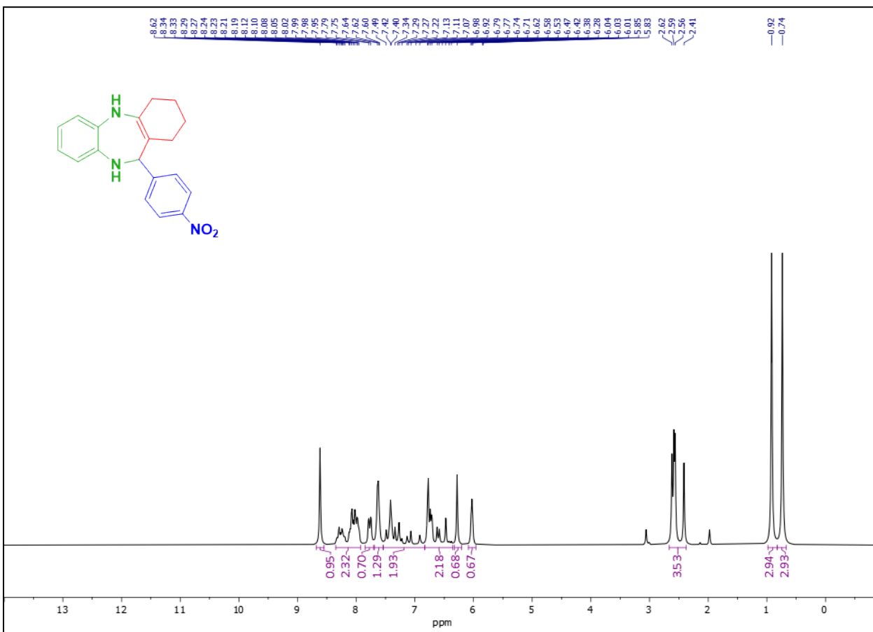
1 H-NMR spectra of 4c
