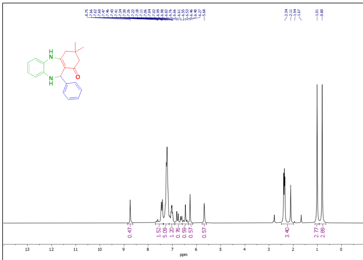
1 H-NMR spectra of 4a
