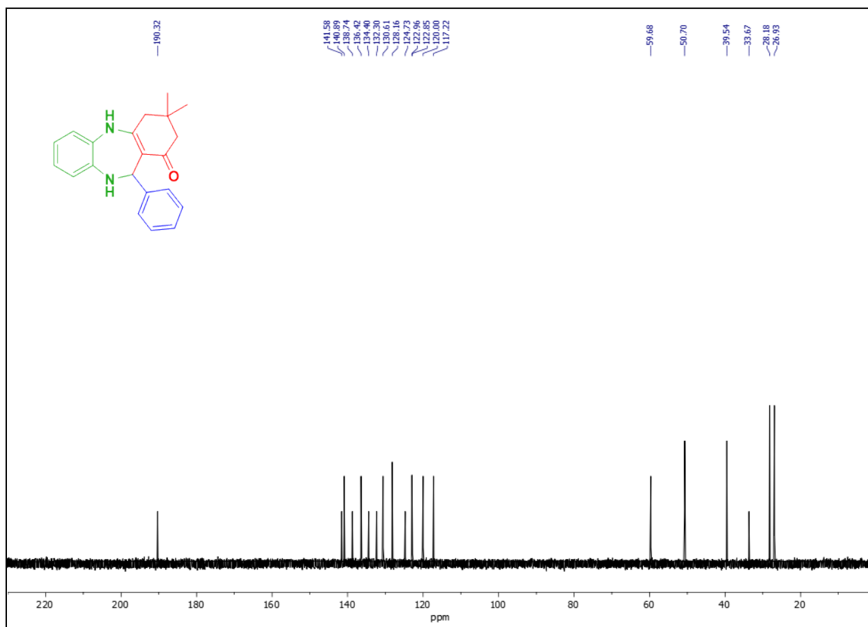
^{13}\text{C} -NMR spectra of 4a
