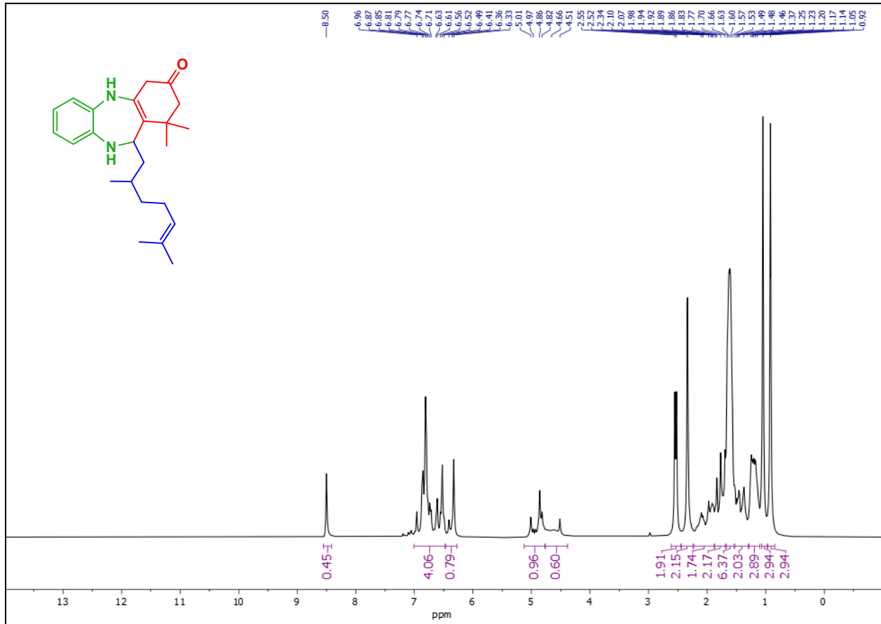
1 H-NMR spectra of 4n
