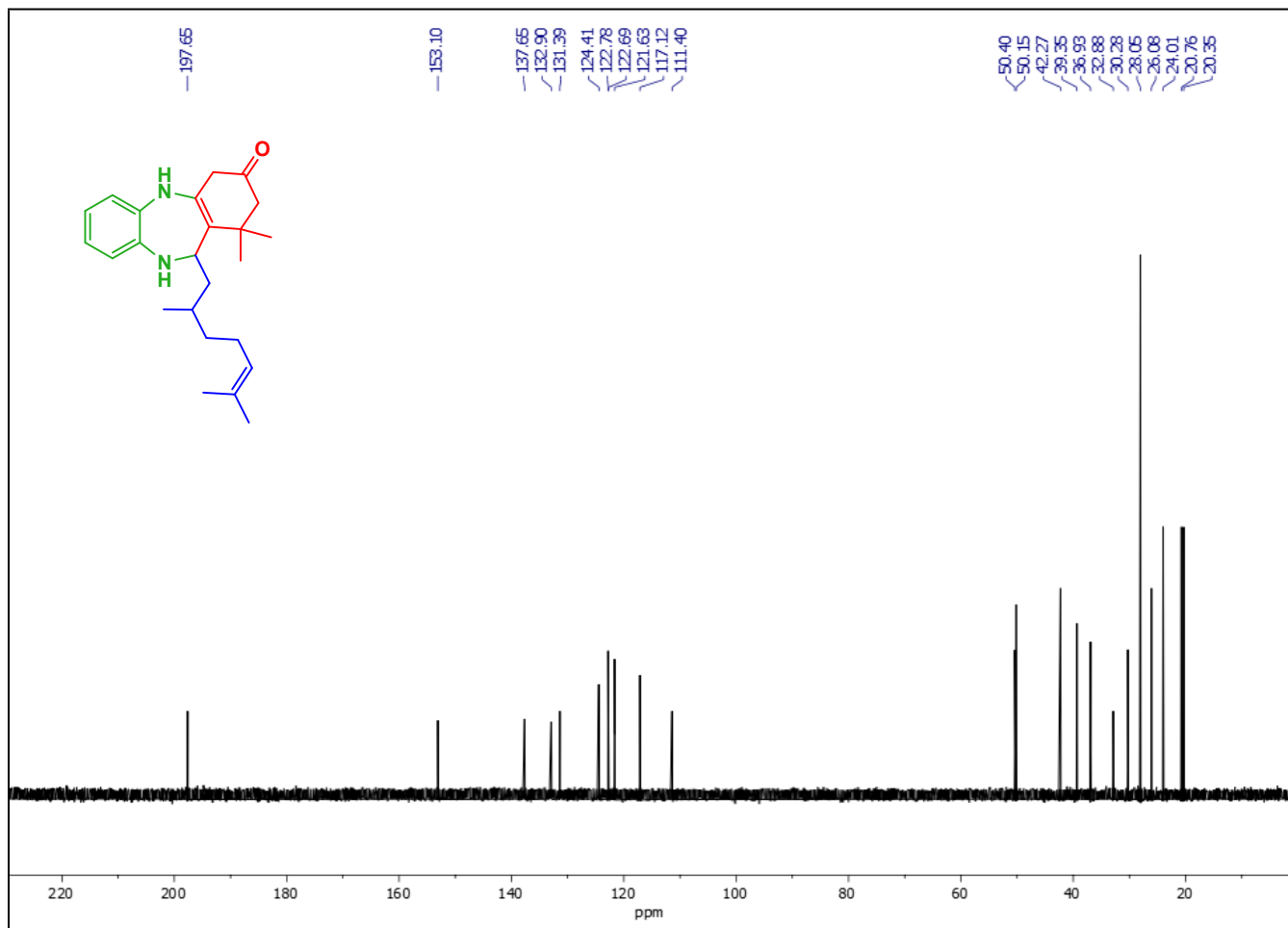
13 C-NMR spectra of 4n
