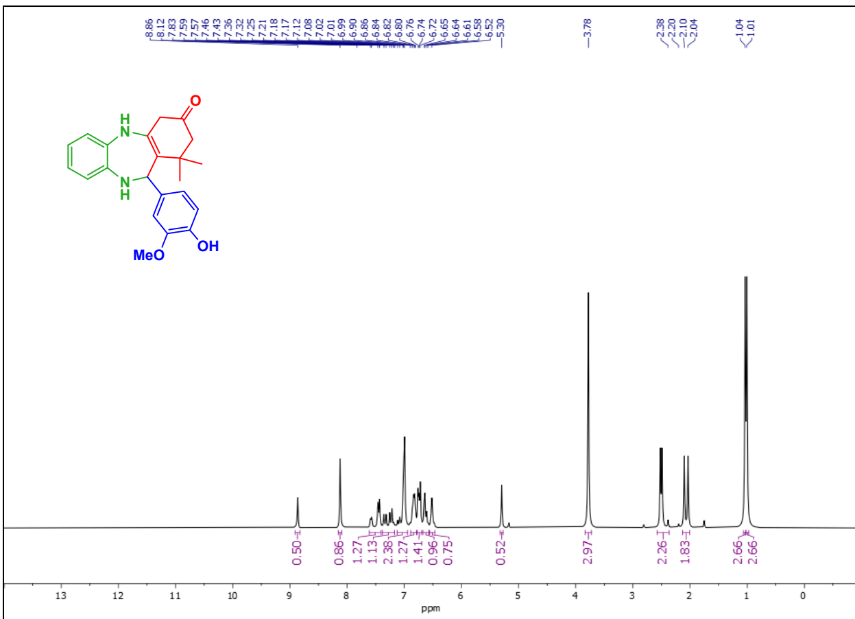
1 H-NMR spectra of 4i
