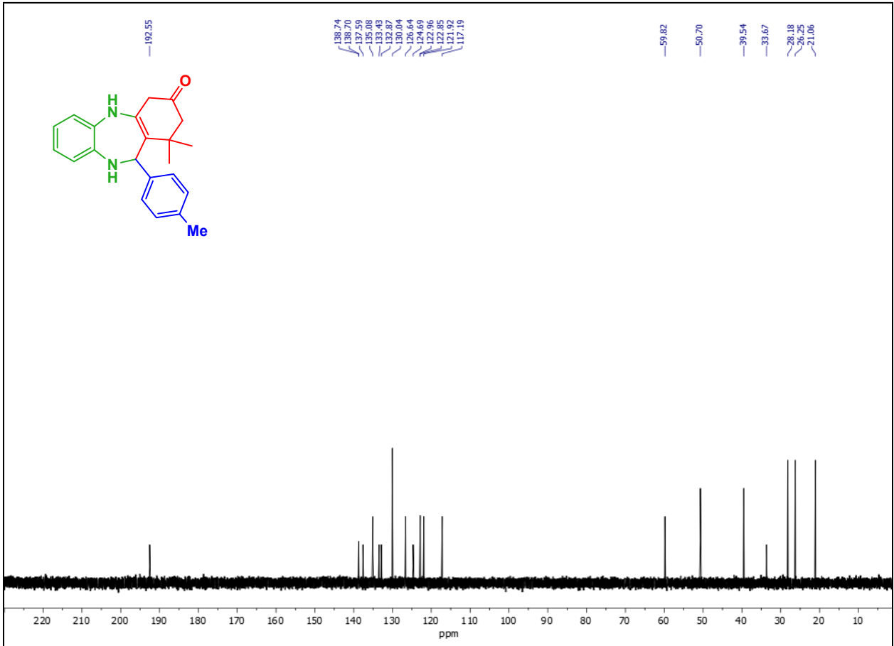
13 C-NMR spectra of 4k
