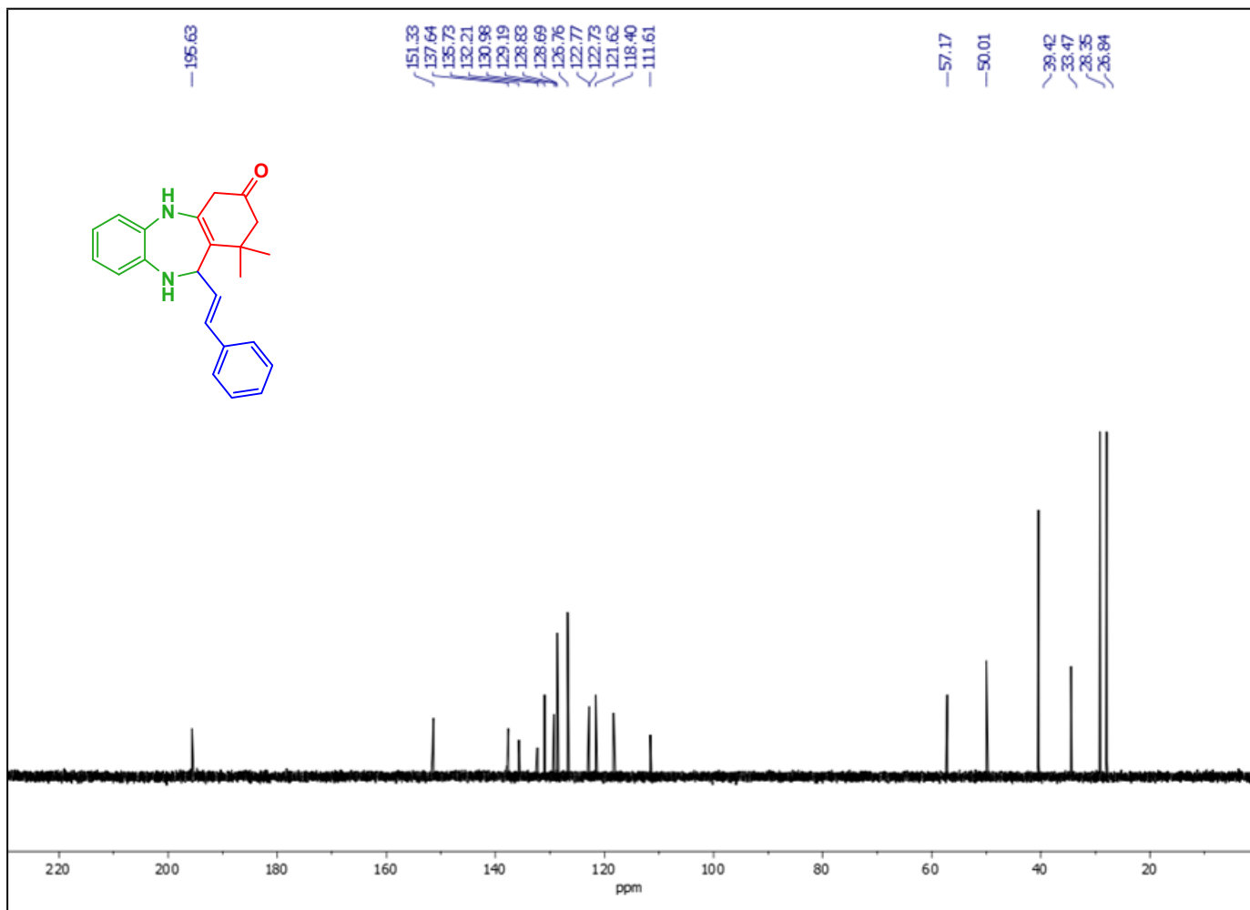
13 C-NMR spectra of 4l
