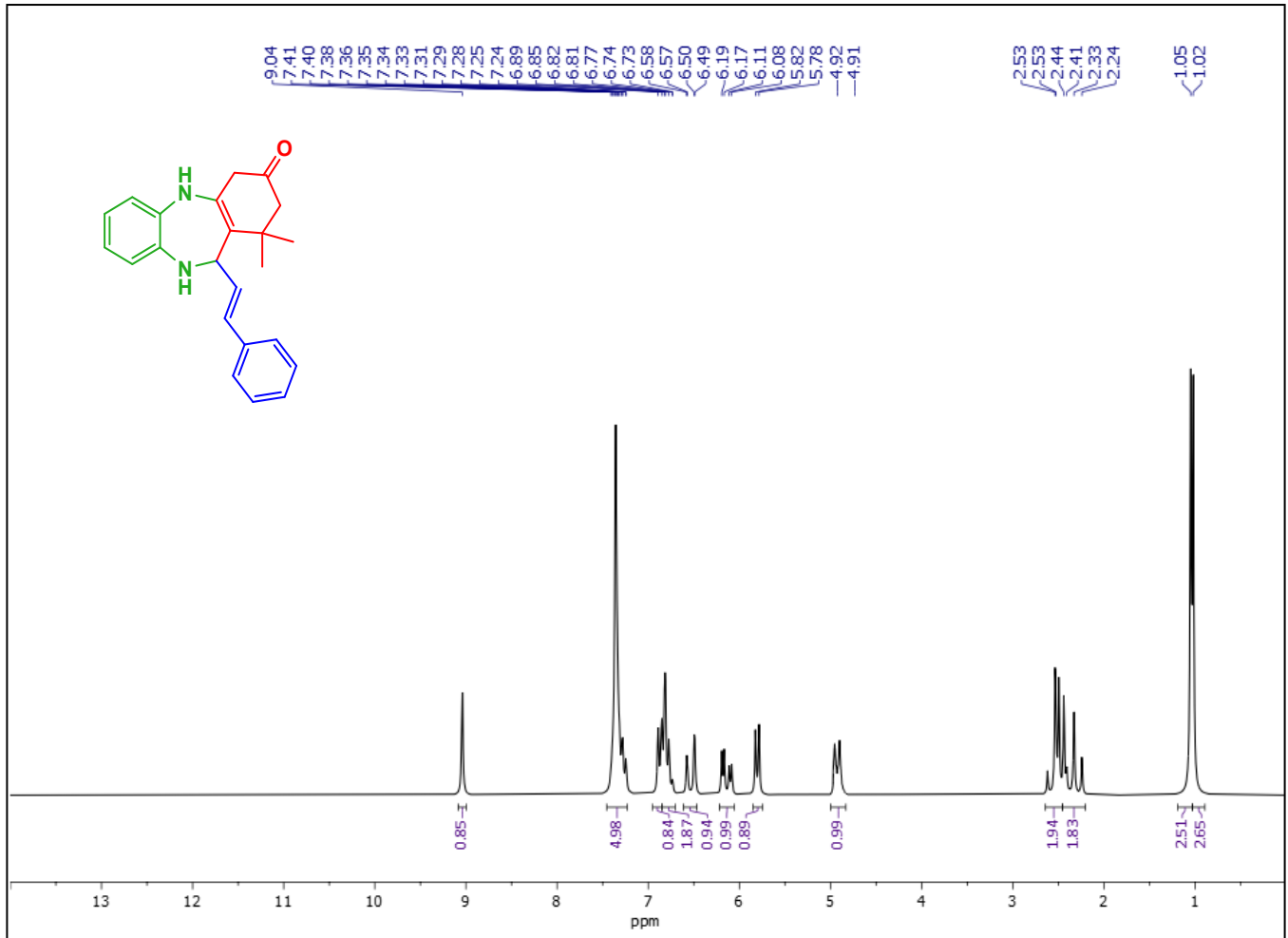
^1\text{H-NMR} spectra of 4l
