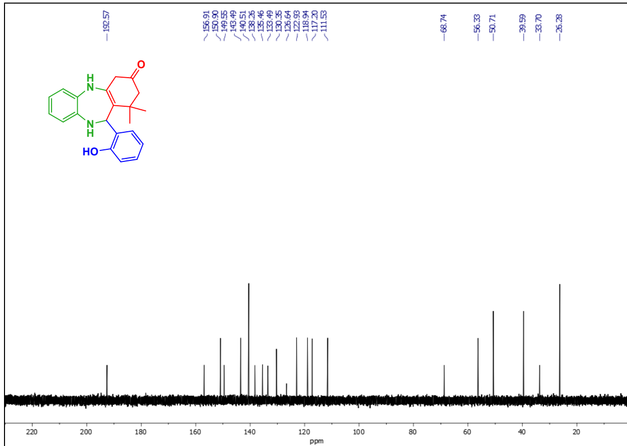
13 C-NMR spectra of 4b
