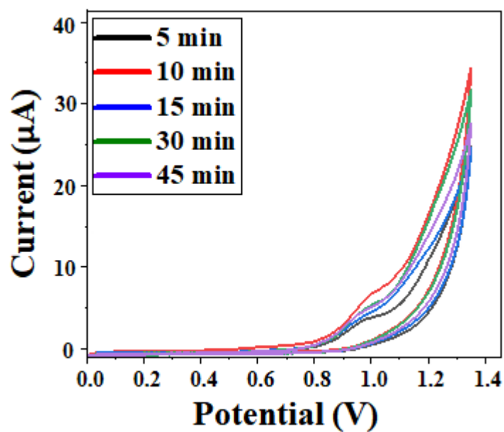
Fig. S1: CV for optimization of nanoparticles amount to transform PGE.
