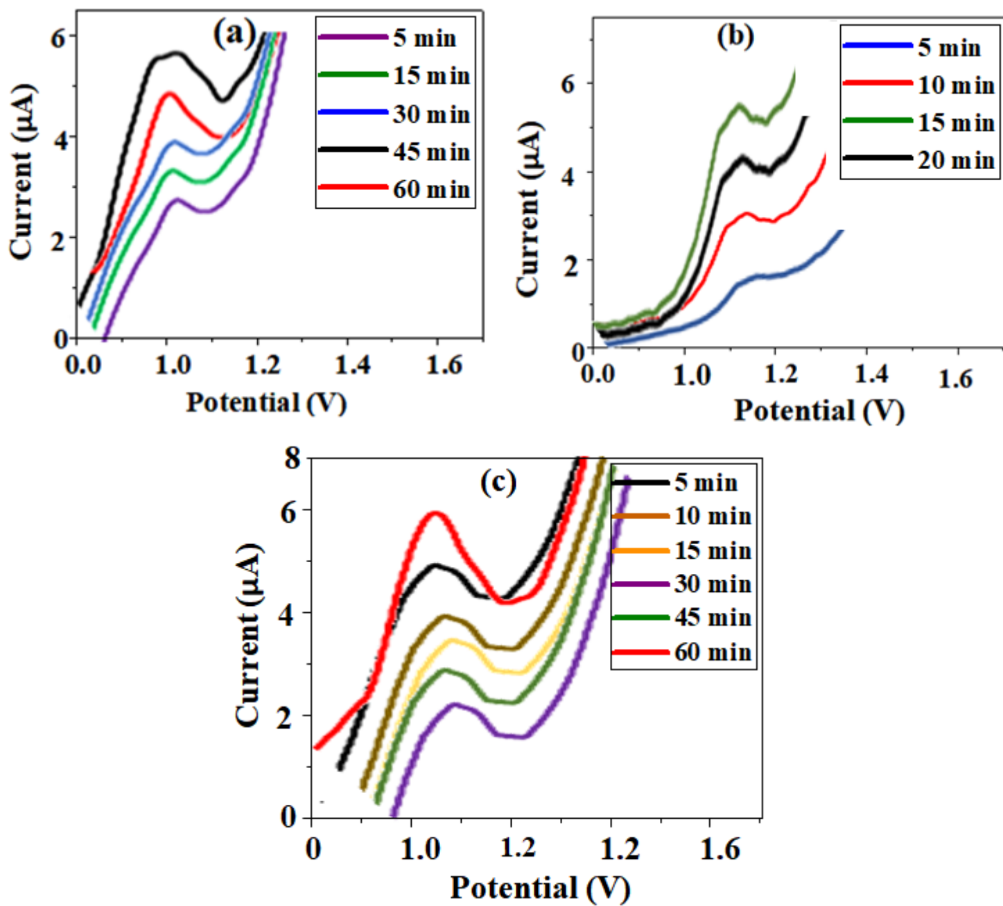
Fig. S2: DPV for optimizations (a) Electrode modification time with nanoparticles, (b) Electrode modification time with nanoparticles and enzymes, (c) Time incubation for same concentration of drug.
