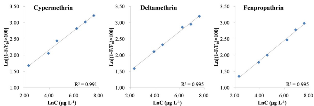
Figure S4 The standard curves of the relationship between CPs concentration and fluorescence intensity
