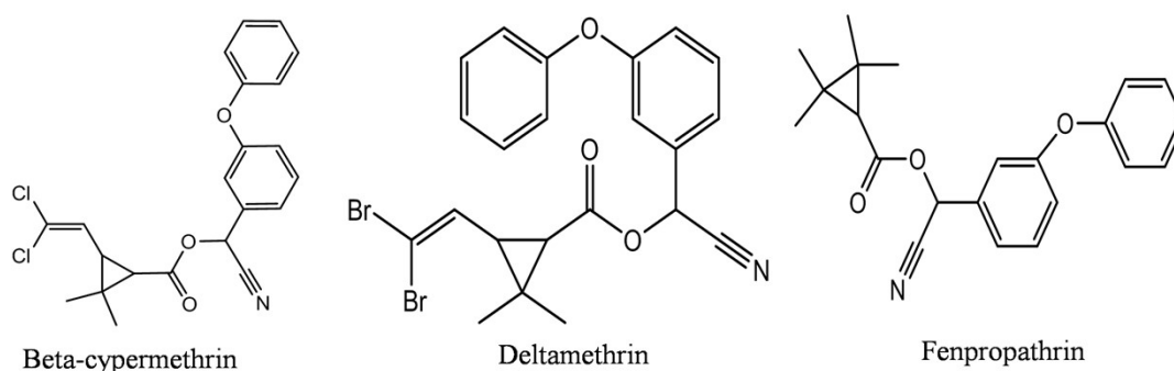
Figure S1 The molecular structures of cypermethrin, deltamethrin and fenpropathrin
