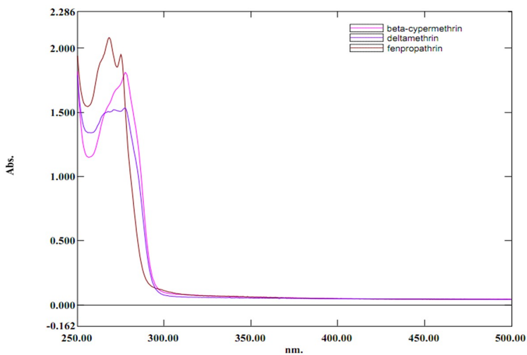
Figure S2 UV-vis absorption spectra of cypermethrin, deltamethrin and fenpropathrin ( 1 \text{ mg mL}^{-1} )
