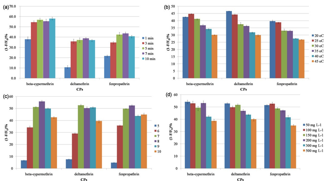
Figure S3 Optimization of experimental conditions. reaction time (a), reaction temperature (b), pH value (c) and concentration of benzothiazole-CDs (d) (n=5)
