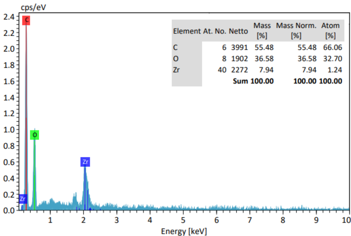
Figure S 1. EDS analysis of Zr-UiO-67.
