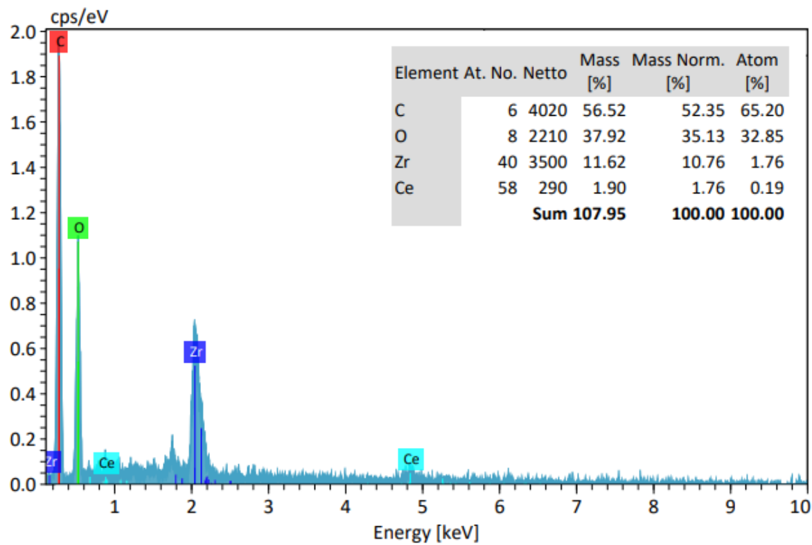
Figure S 2. EDS analysis of Zr/Ce-UiO-67(1:3).
