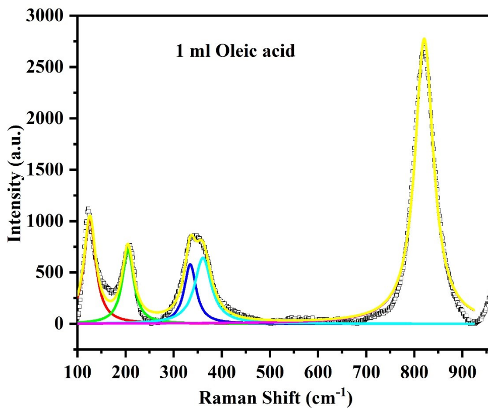
S2. Deconvoluted Raman spectra of \text{BiVO}_4 sample synthesized with 1 ml of oleic acid.
