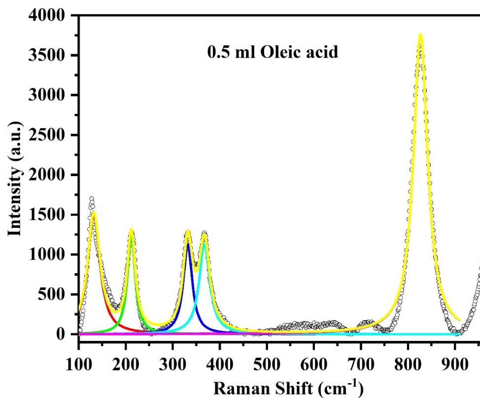
S1. Deconvoluted Raman spectra of BiVO 4 sample synthesized with 0.5 ml of oleic acid.
