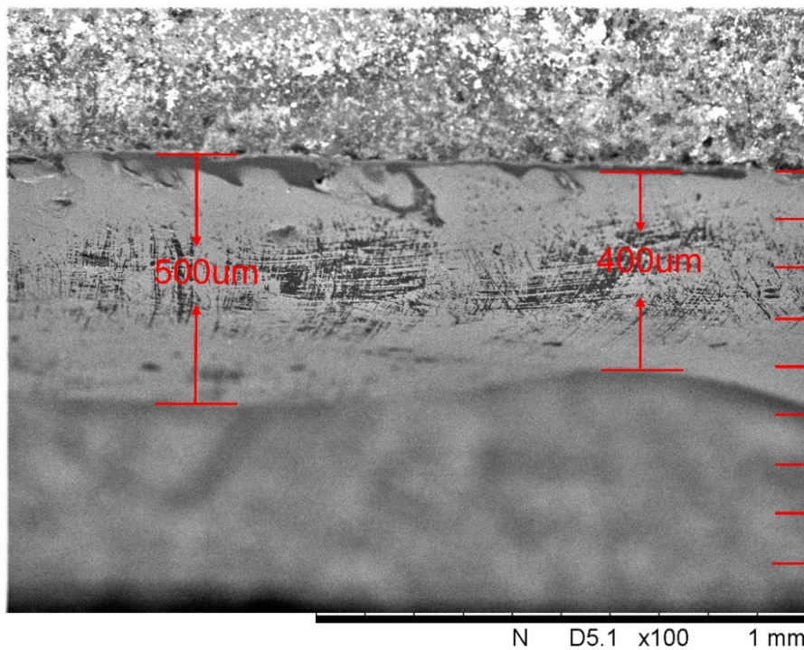
Figure S4. The thickness of the electrolyte thin film.
