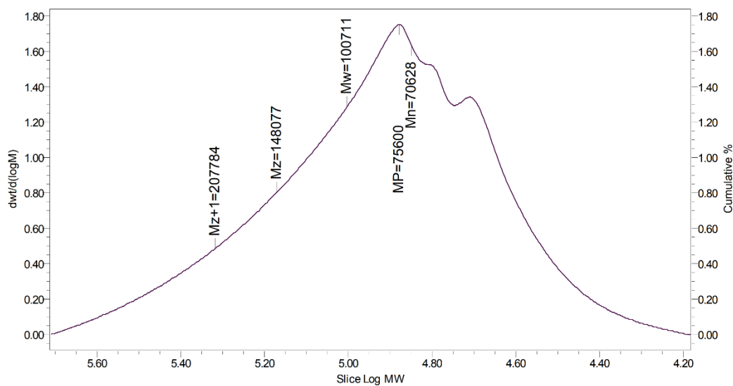
Figure S1. The GPC curve for polymer 6-HW.
