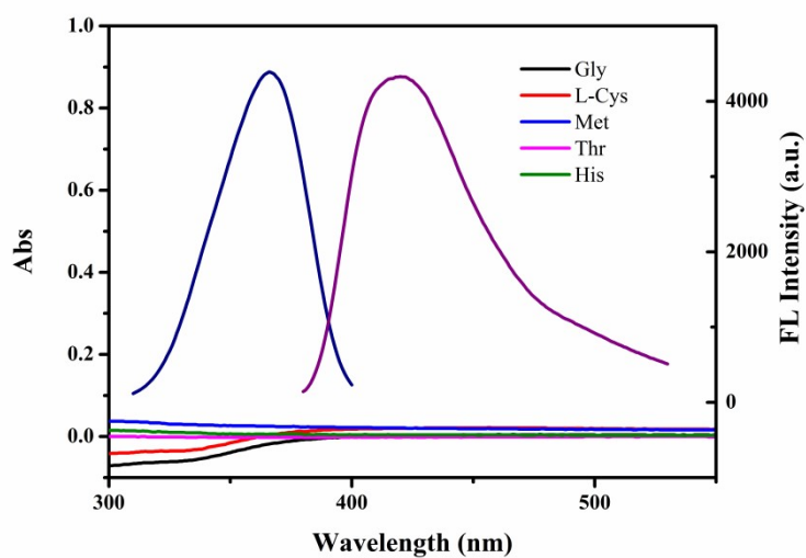
Fig. S1 UV-Vis spectra of amino acids and the fluorescence excitation and emission spectra of EGCG-Cu NCs.(amino acids: glycine, L-cysteine, methionine, threonine, histidine) .
