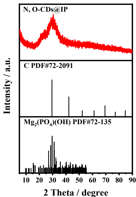
Figure S1. XRD patterns of CDs@Phosphate composite and the standard diffraction pattern of C (JCPDS Card No. 72-2091) and Mg 2 (PO 4 )(OH) (JCPDS Card No. 72-135).
