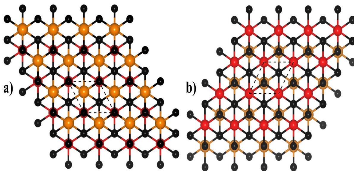
Fig. S3. (a, b) Top and Bottom view of BBA1 stacking of v-HS PtS 2 /ZrS 2
