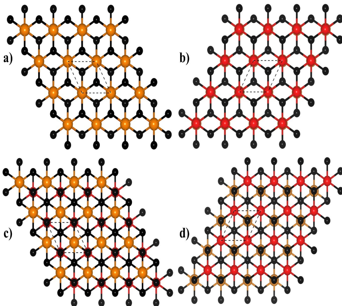
Fig. S1. (a, b) Top and Bottom view of ABB1 stacking of v-HS PtS 2 /ZrS 2 (c, d) Top and Bottom view BAB stacking of v-HS PtS 2 /ZrS 2
