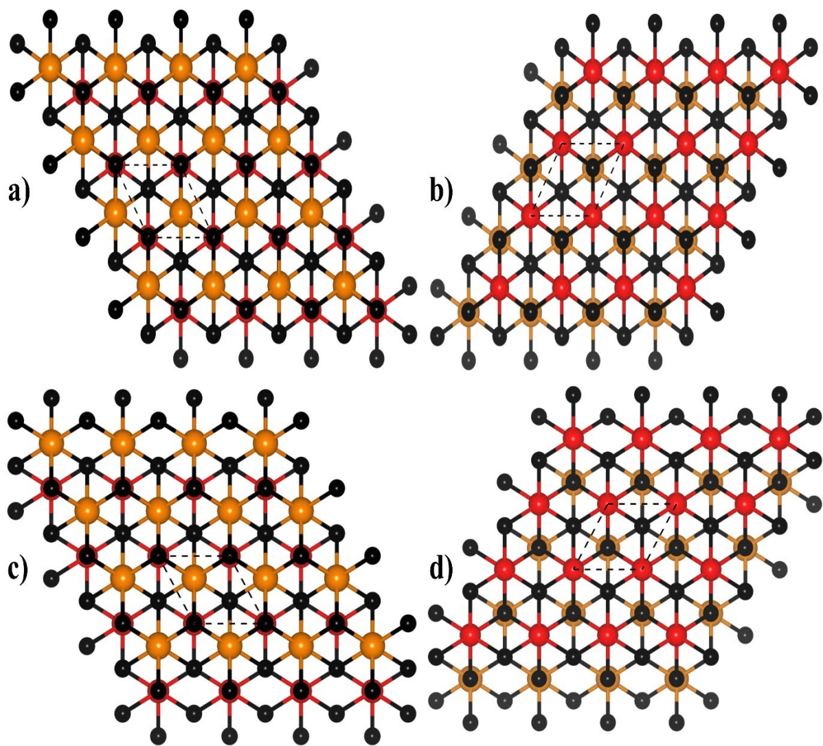
Fig. S2. (a, b) Top and Bottom view of BAB1 stacking of v-HS PtS 2 /ZrS 2 (c, d) Top and Bottom view BBA stacking of v-HS PtS 2 /ZrS 2
