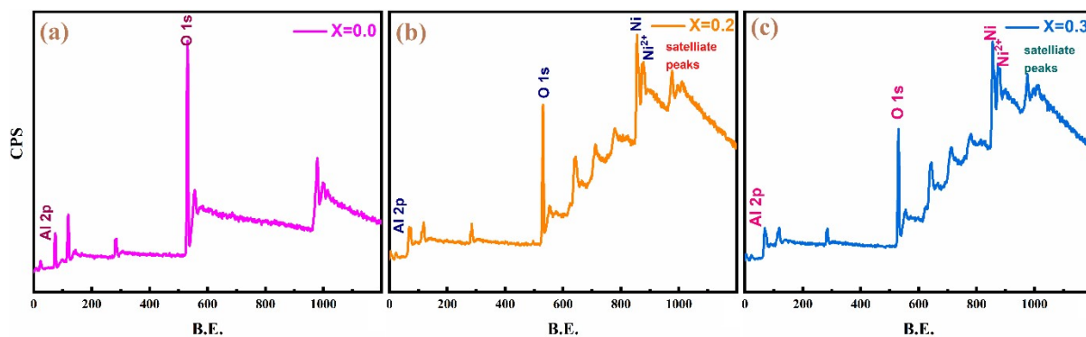
Fig. S1 XPS survey scan of undoped and doped aluminum oxide nanoparticles.
