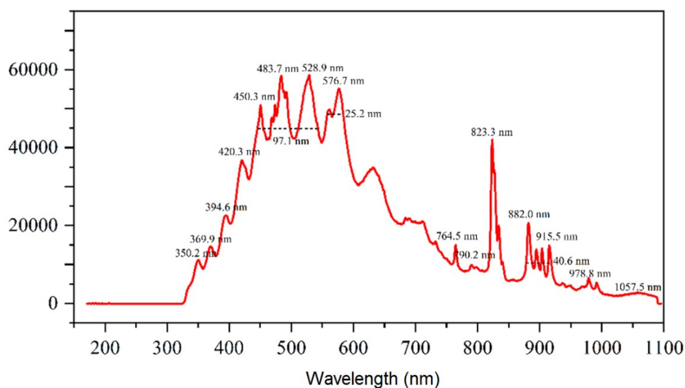
Fig. S1. Emission spectrum of a 300 W xenon lamp equipped with a filter up to 420 nm.
