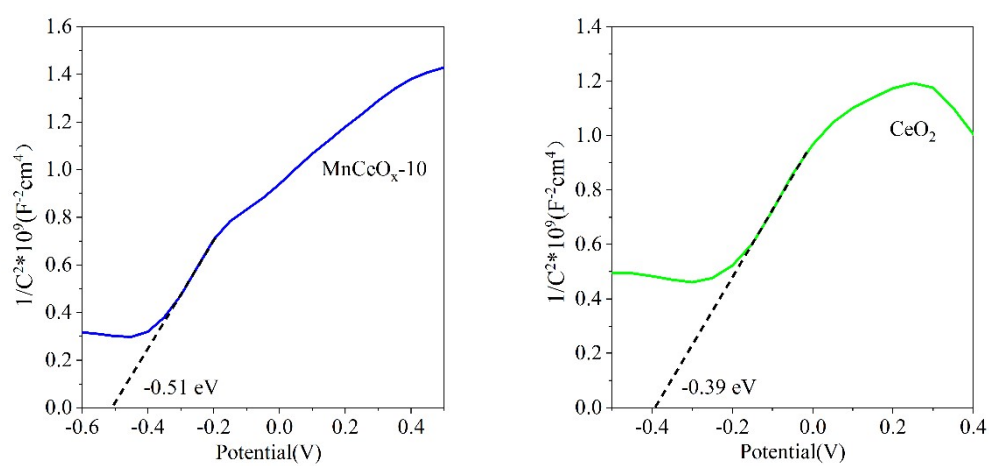
Fig. S2. Mott-Schottky diagrams of pure CeO 2 and MnCeO x -10 samples.
