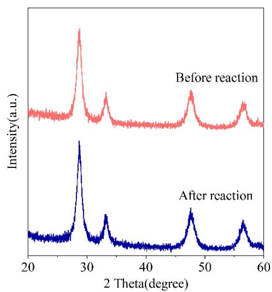
Fig. S3. XRD patterns of MnCeO x -10 catalyst before and after reaction.
