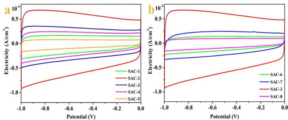
Figure S3 CV curves of SAC samples at 100 mV/s
