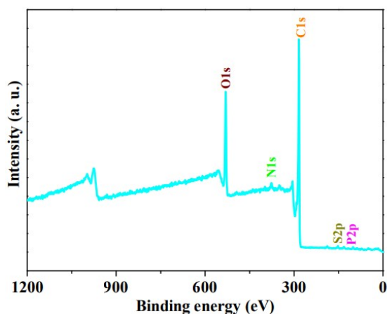
Figure S1 Survey spectrum and high-resolution spectra of SAC-2
