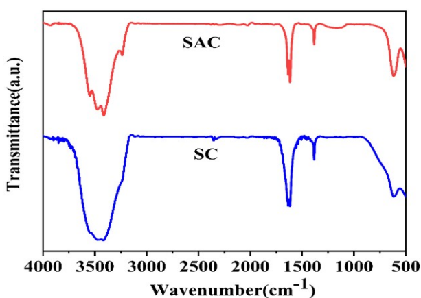
Figure S2 FT-IR spectra of SAC-2 and SC
