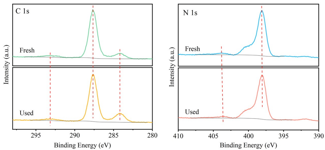
Figure S1. (a) C 1s and (b) N 1s XPS spectra of 10% BgM before and after used.
