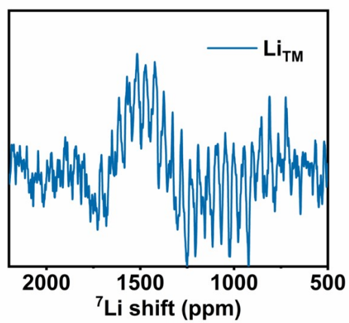
Fig. S4 {}^7\text{Li} ss-NMR of KLMO.
