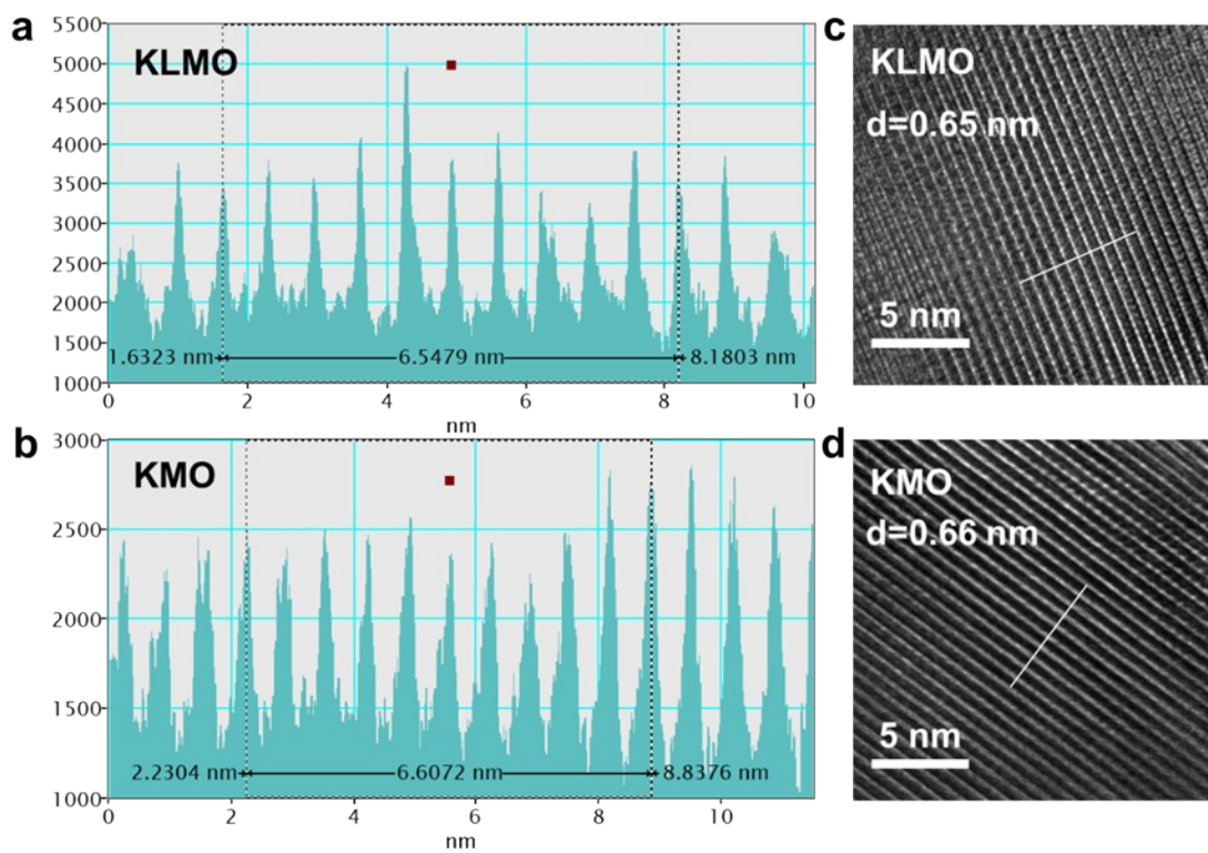
Fig. S3 The intensity line profiles of signals corresponding to (a) KLMO and (b) KMO from (c-d) HRTEM images.
