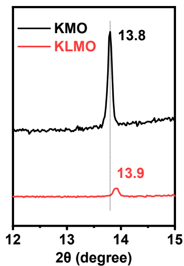
Fig. S1. Enlarged XRD profiles of (a) KMO and (d) KLMO
