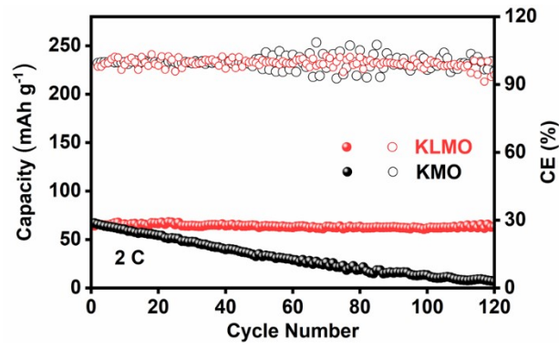
Fig. S7 Cycle stabilities of KMO and KLMO at 2C.
