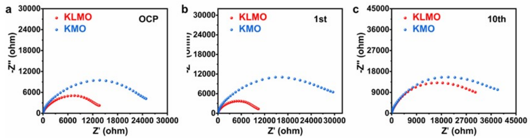
Fig. S6 EIS plots of KLMO and KMO (a) at open-circuit voltage, (b) after 1 cycle, and (c) 10 cycles.
