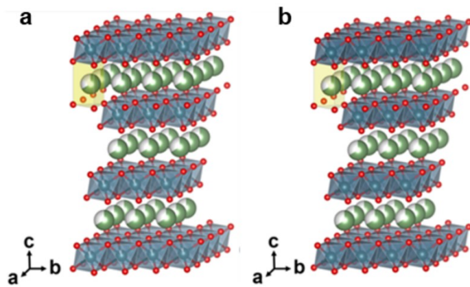
Fig. S2 Crystal structures of (a) KLMO and (b) KMO along the c-axis.
