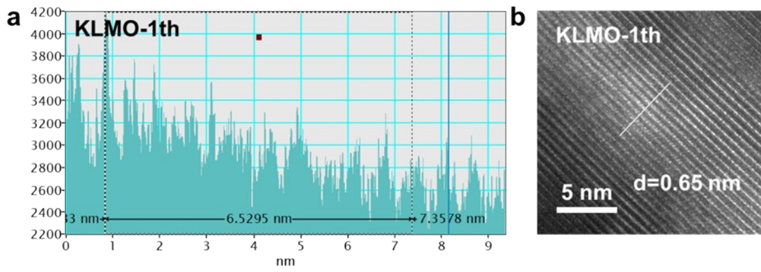
Fig. S5 The intensity line profiles of signals corresponding to (a) KLMO after one cycle from (b) HRTEM image.
