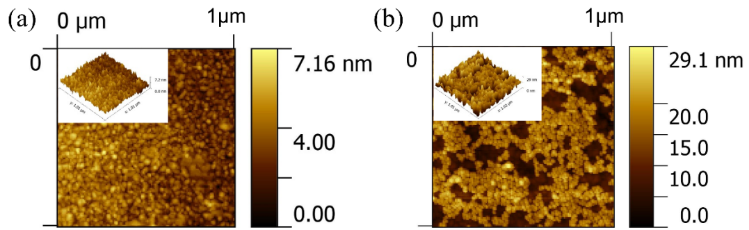
Figure S3 Two-dimensional AFM images of (a) GF and (b) GF-AuNP. Insets are three-dimensional AFM images of (a) GF and (b) GF-AuNP.
