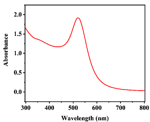
Figure S2 UV-VIS spectrum of AuNPs solution.
