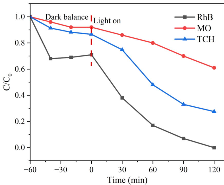
Fig. S1 Photocatalytic degradation curves of RhB, MO and TCH over P-Si/ZnO-90°C after 120 min of UV-Vis light irradiation. Experimental conditions: Substrate, 5 mg L -1
