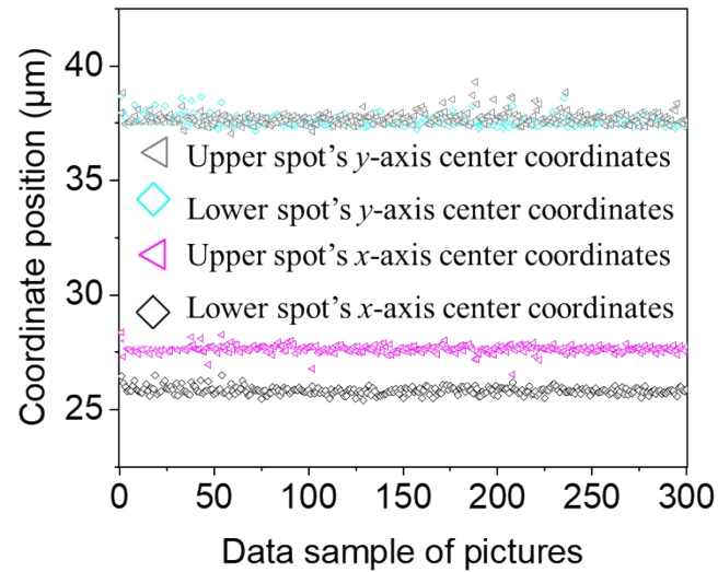
Fig. S5 XY center coordinates corresponding to the two strong spots in the vortex pair beam in the case of m_1 = 1, m_2 = 1 .
