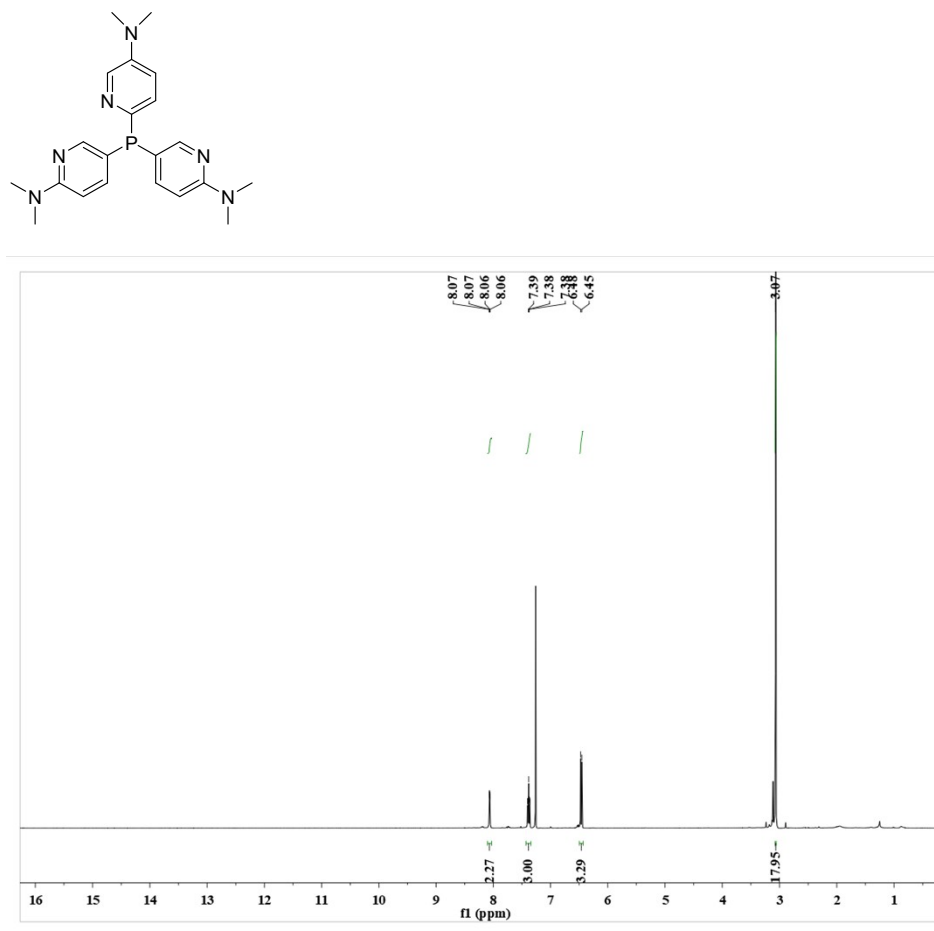
Figure S17 1 H NMR of tri(4-N,N-dimethyl-pyridyl)phosphine (L9)
