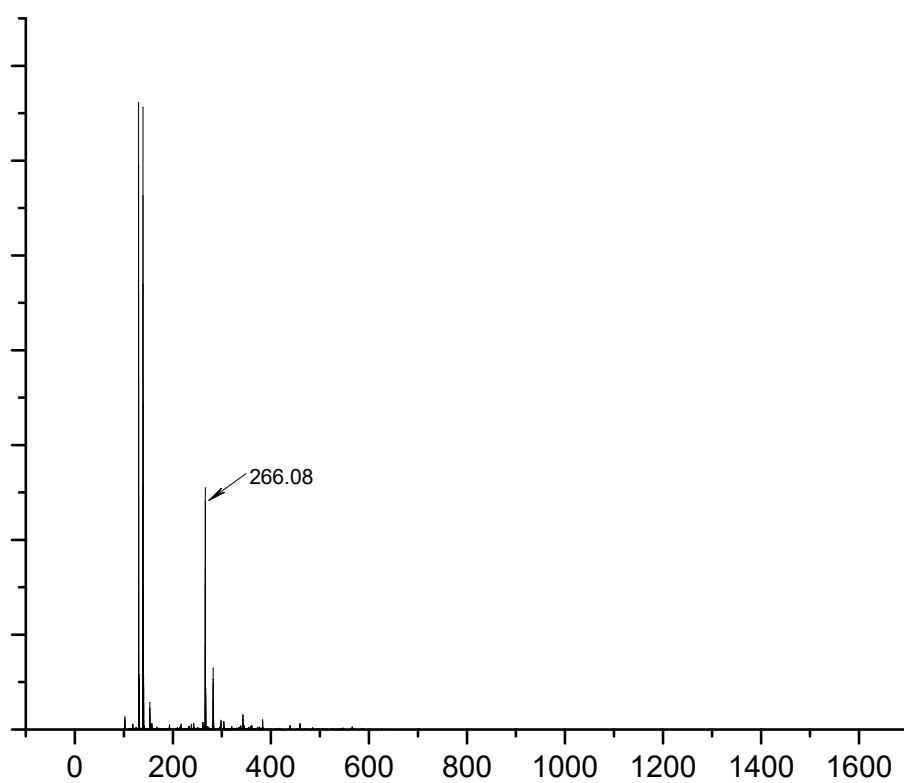
Figure S4 Electrospray mass spectrometry of tri(3-pyridyl)phosphine (L5)
