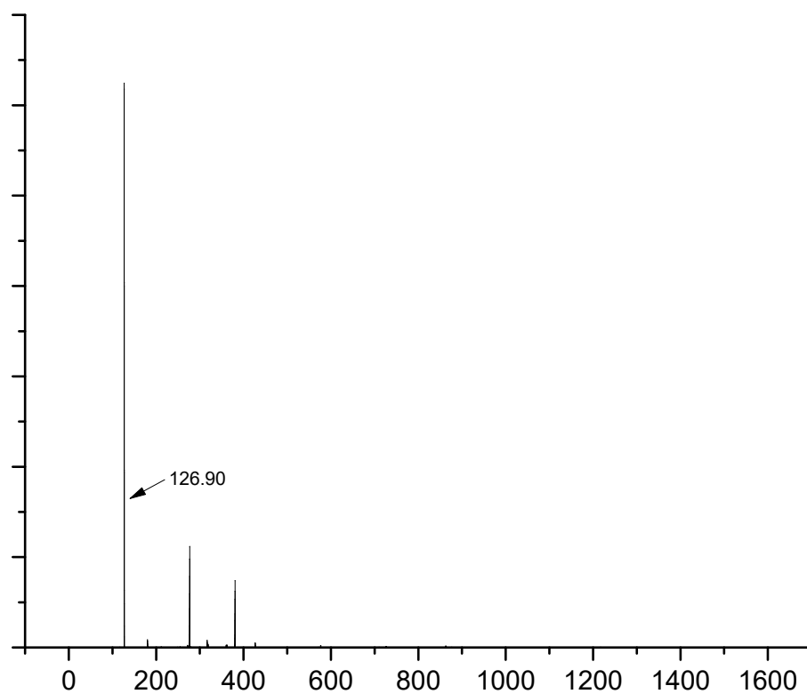
Figure S25 Electrospray mass spectrometry of tri(1-propylpyridinium iodide)phosphine (L5-1)-I - .
