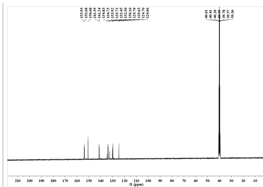
Figure S6 13 C NMR of di(3-pyridyl)phenylphosphine (L6)
