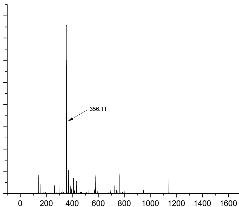
Figure S16 Electrospray mass spectrometry of tri(4-methoxypyridyl)phosphine (L8)
