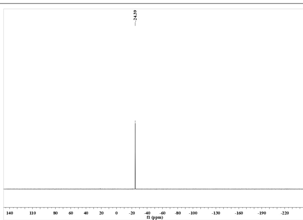
Figure S3 ^{31}\text{P} NMR of tri(3-pyridyl)phosphine (L5)
