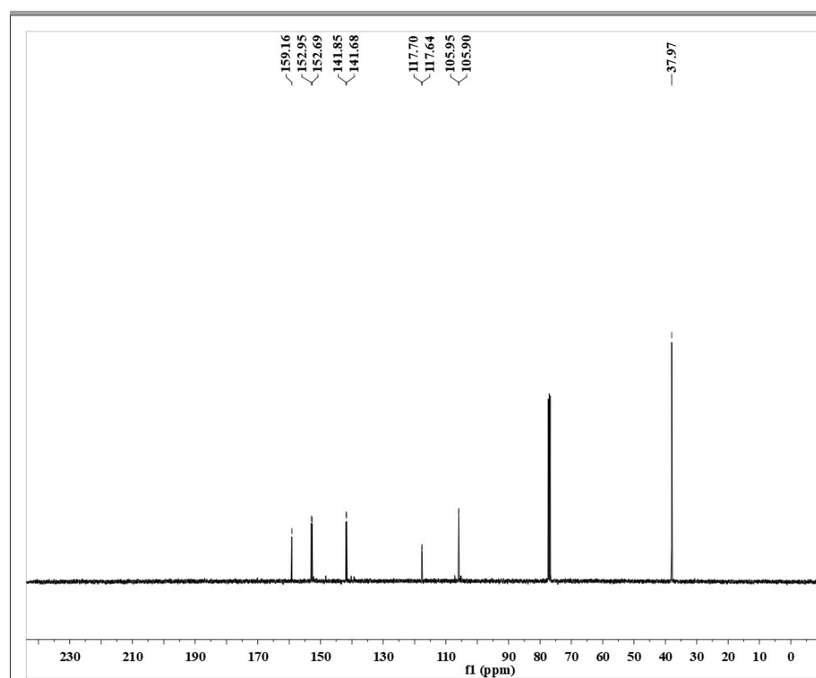
Figure S18 13 C NMR of tri(4-N,N-dimethyl-pyridyl)phosphine (L9)
