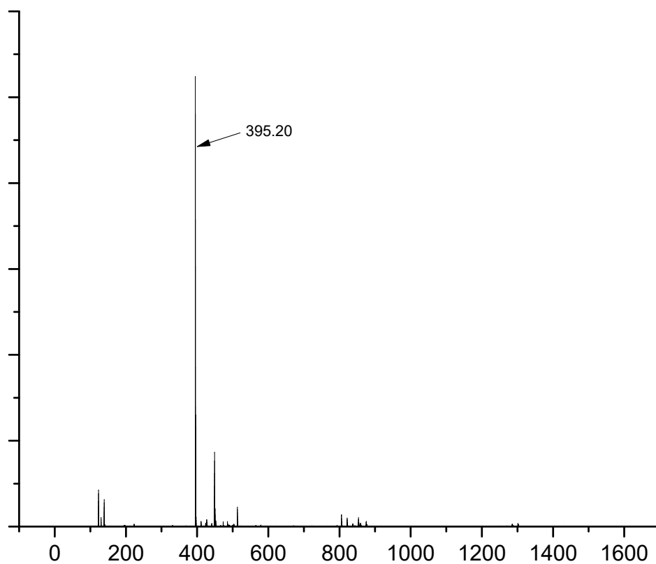
Figure S20 Electrospray mass spectrometry of tri(4-N,N-dimethyl-pyridyl)phosphine
