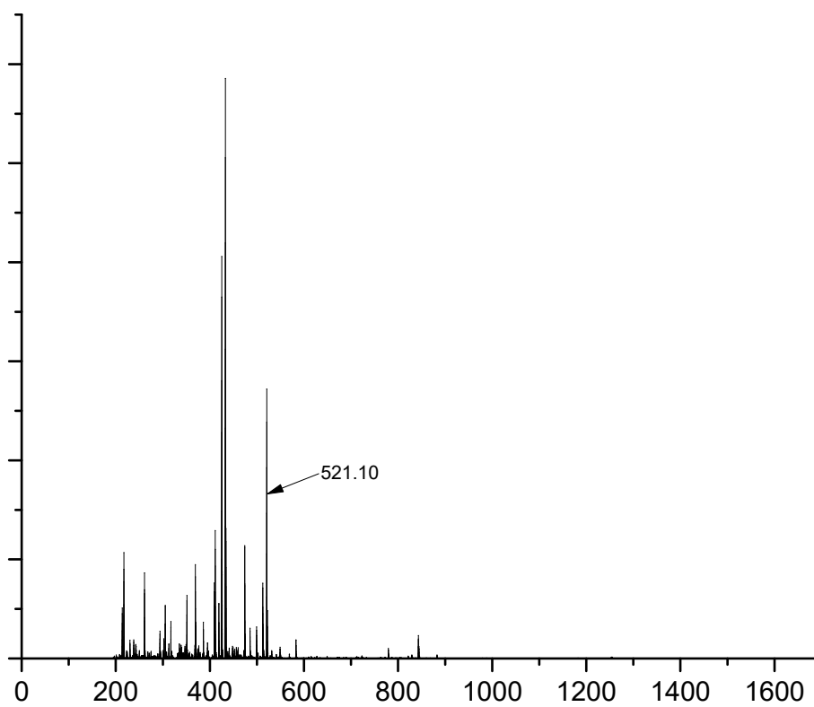
Figure S24 Electrospray mass spectrometry of tri(1-propylpyridinium iodide)phosphine (L5-1)- \text{C}_{24}\text{H}_{32}\text{IN}_3\text{P}^+
