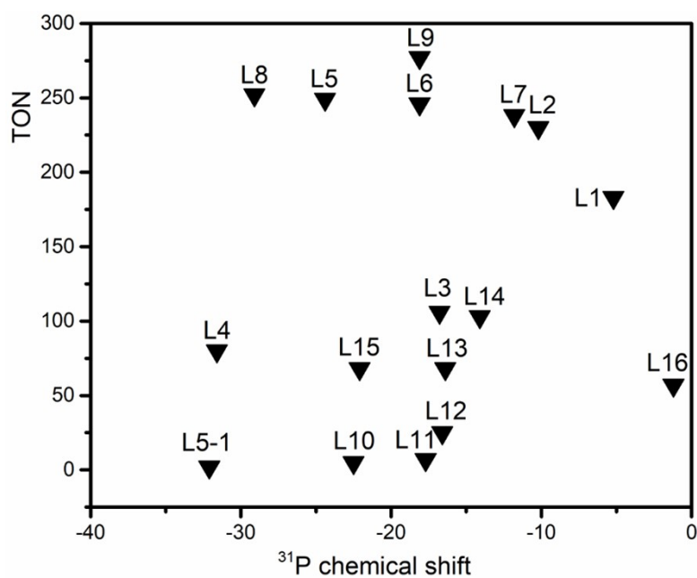
Figure S28. The 31 P Chemical shift of different ligands VS TON of the reactions
