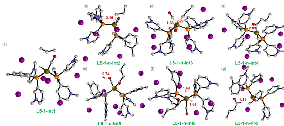
Figure S27 The results of the optimized structures based on Ir-L5-1.
