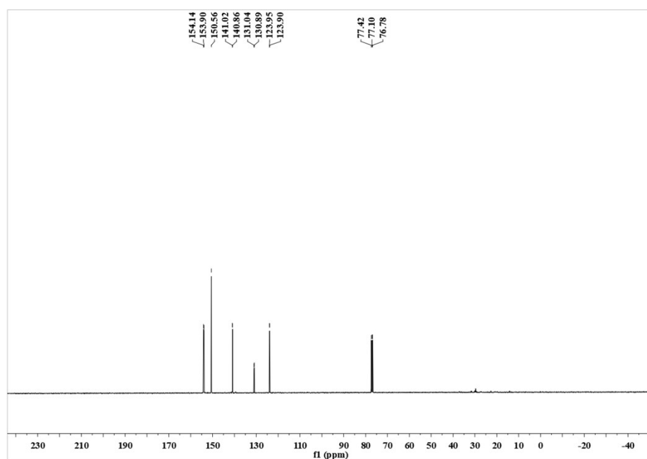
Figure S2 13 C NMR of tri(3-pyridyl)phosphine (L5)
