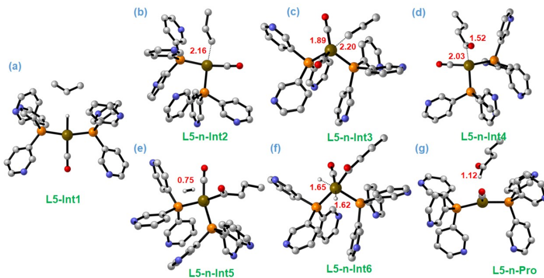
Figure S26 The results of the optimized structures based on Ir-L5.
