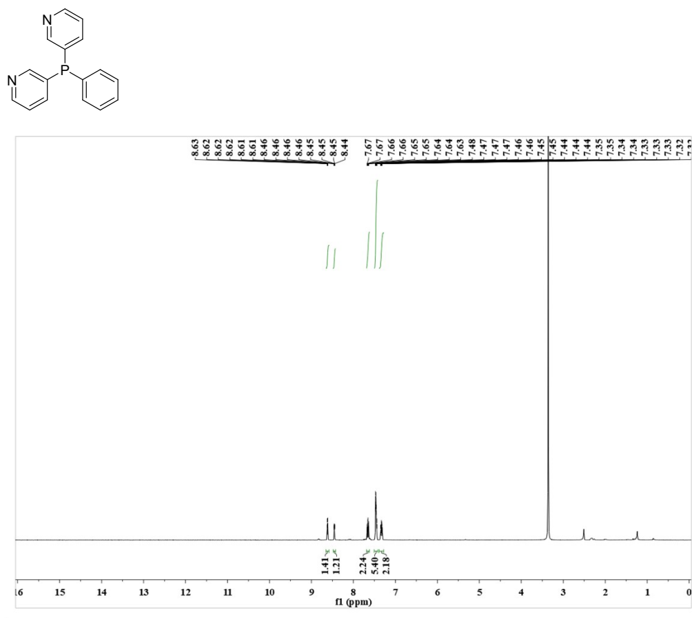
Figure S5 1 H NMR of di(3-pyridyl)phenylphosphine (L6)
