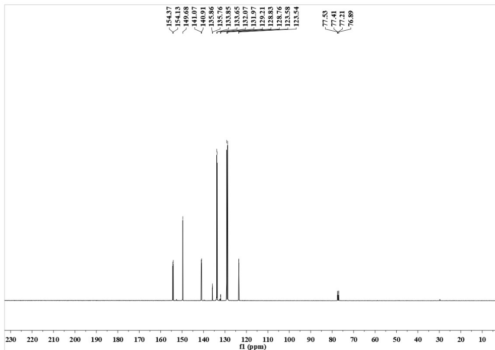
Figure S10 13 C NMR of diphenyl(3-pyridyl)phosphine (L7)
