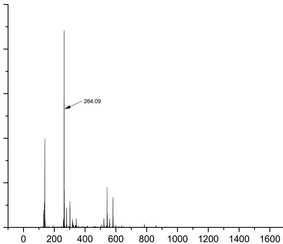
Figure S12 Electrospray mass spectrometry of diphenyl(3-pyridyl)phosphine (L7)
