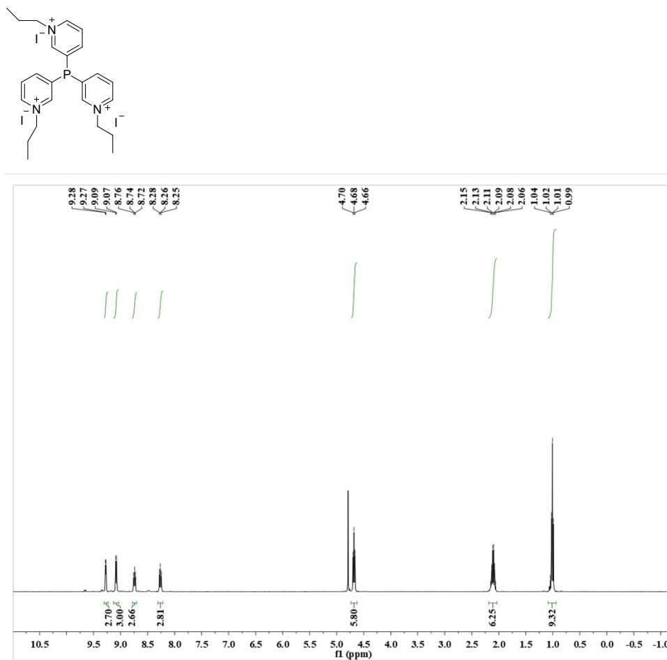
Figure S21 1 H NMR of tri(1-propylpyridinium iodide)phosphine (L5-1)
