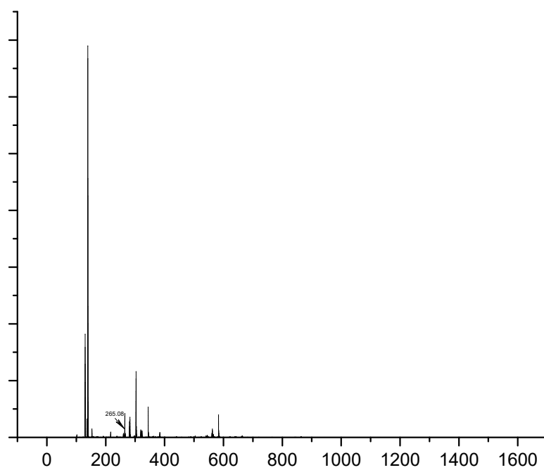
Figure S8 Electrospray mass spectrometry of di(3-pyridyl)phenylphosphine (L6)
