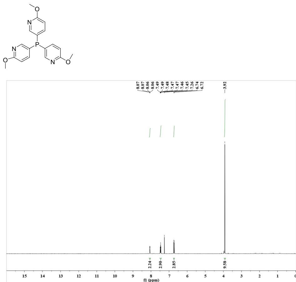
Figure S13 1 H NMR of tri(4-methoxypyridyl)phosphine (L8)
