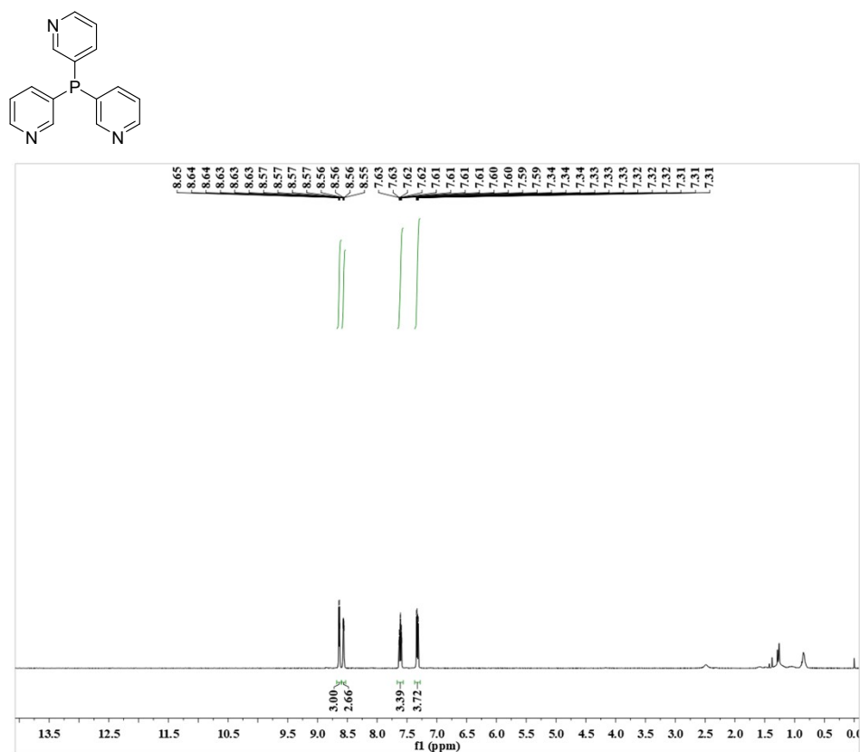
Figure S1 1 H NMR of tri(3-pyridyl)phosphine (L5)
