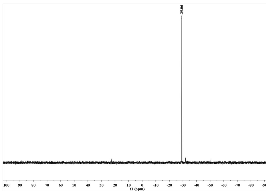
Figure S15 ^{31}\text{P} NMR of tri(4-methoxypyridyl)phosphine (L8)
