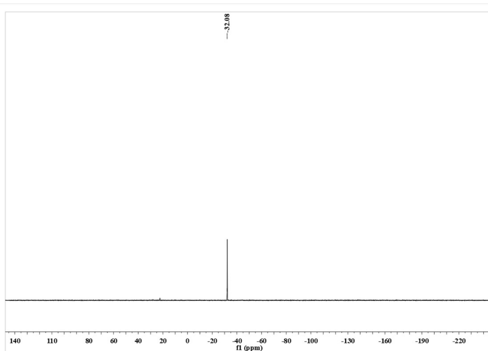
Figure S23 ^{31}\text{P} NMR of tri(1-propylpyridinium iodide)phosphine (L5-1)
