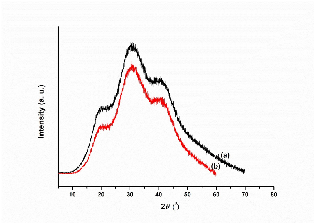
Supplementary Fig 1. X-ray diffractograms of fucoidan (a) and fucoidan-PEI complex (b)
