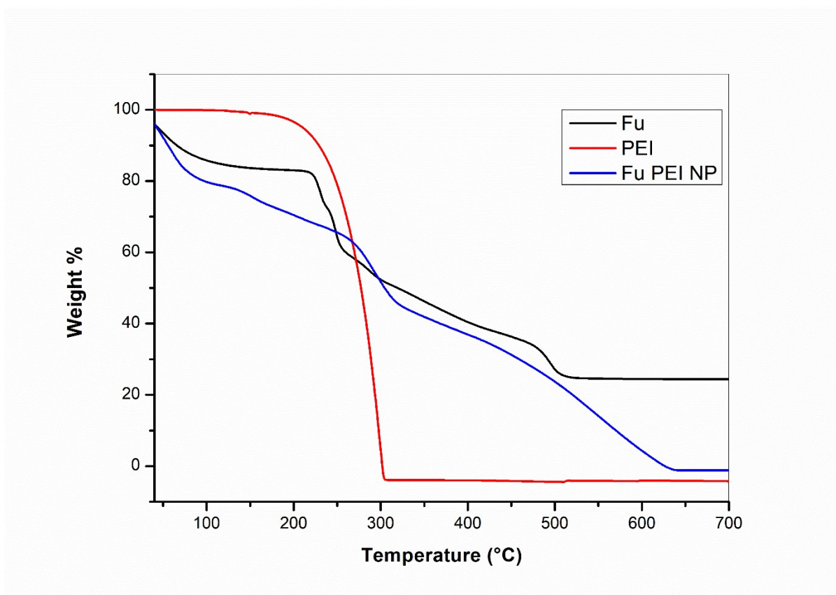
Supplementary Fig 2. TGA curves of fucoidan, PEI and FuNPs
