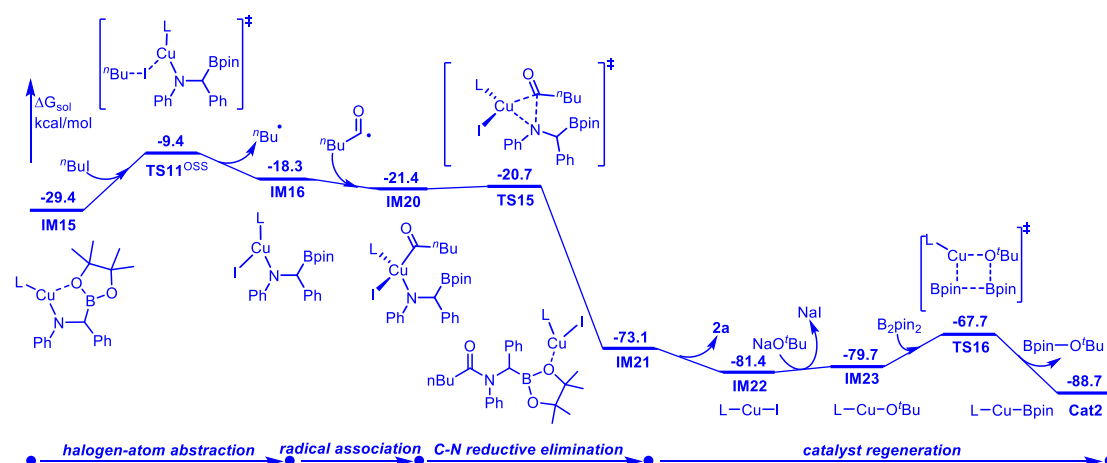
Figure S1. Calculated energy profile leading to \alpha -boryl amide 2a . The Gibbs free energies are given in kcal/mol.
