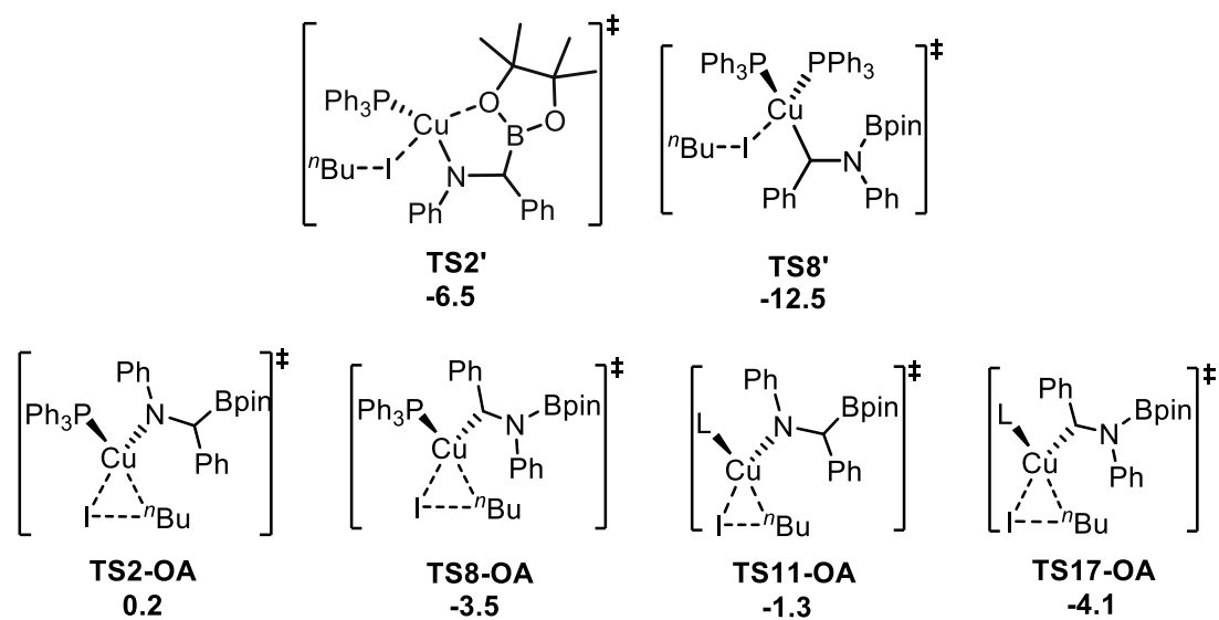
Scheme S2. The alternative pathways of the C-I bond cleavage. The Gibbs free energies are given in kcal/mol.
