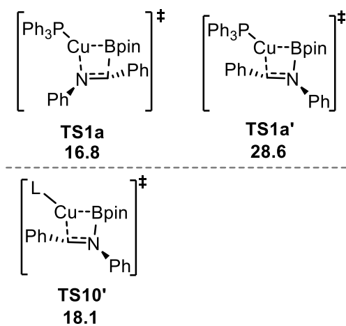
Scheme S1. Other possibilities of the migratory insertion into the Cu-B bond. The Gibbs free energies are given in kcal/mol.
