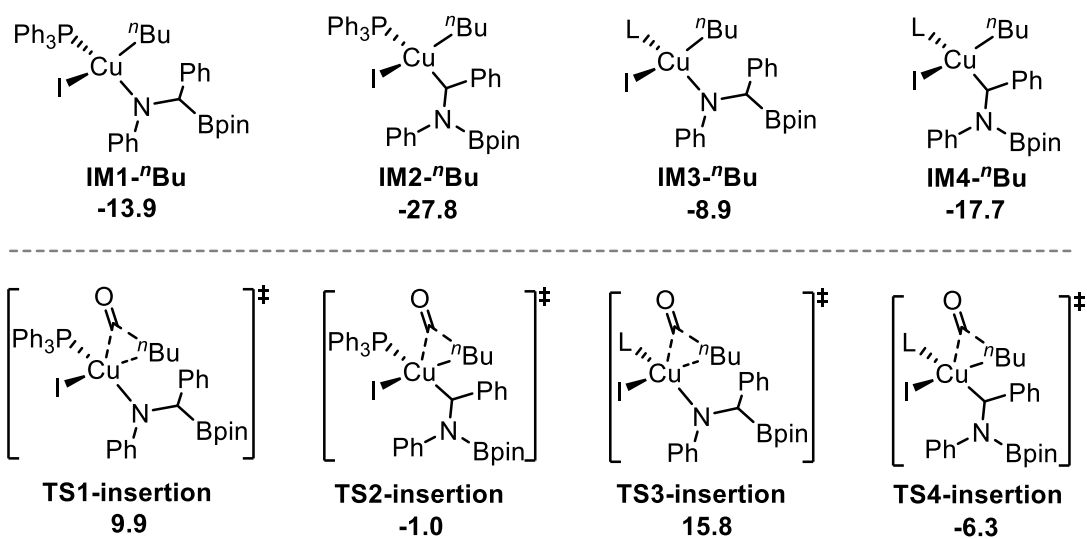
Scheme S4. Other possibilities for the formation of alkylacyl-copper(III) intermediates and amidoacyl-copper(III) intermediates after halogen-atom abstraction. The Gibbs free energies are given in kcal/mol.
