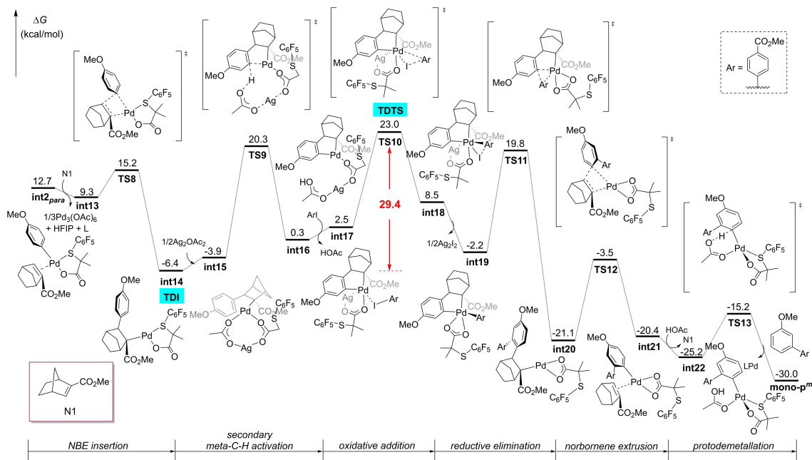
Fig. S6. Free energy profiles for the formation of mono-p''' from primary para -C–H activation in the N1 system.
