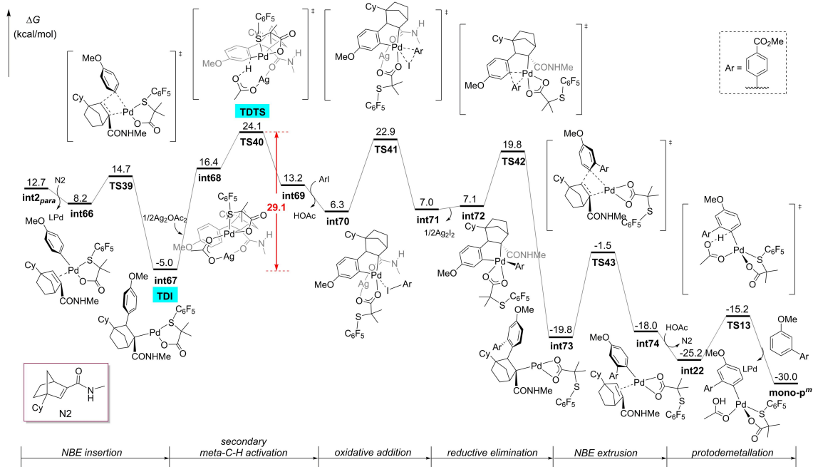
Fig. S11. Free energy profiles for the formation of mono-p''' from primary para -C-H activation in the N2 system.
