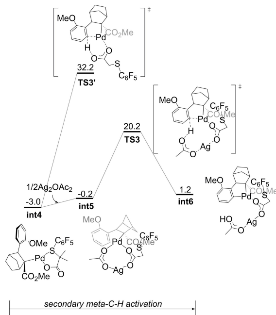
Fig. S4. Free energy profiles for secondary meta -C–H activation catalyzed by monomer Pd and heterodimer Pd-Ag.
