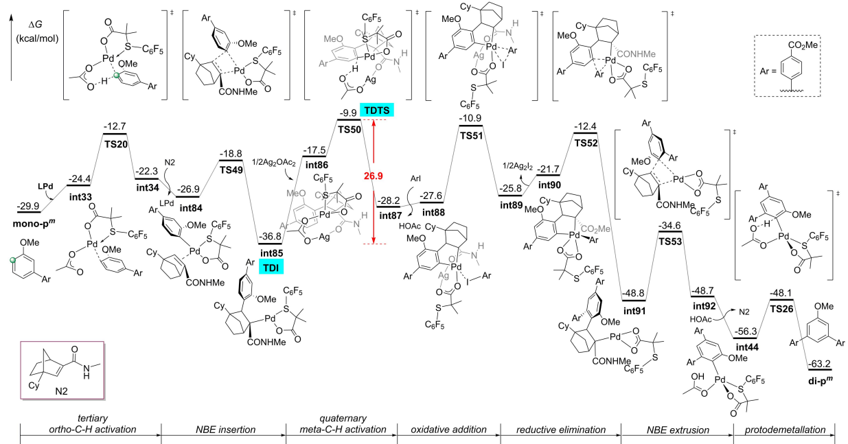
Fig. S13. Free energy profiles for the formation of di-p m from tertiary ortho -C-H activation in the N2 system.
