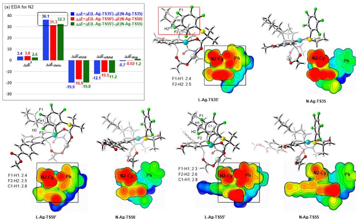
Fig. S16. Energy decomposition analysis in two conformations for secondary and quaternary meta -C–H activation in the N2 system.
