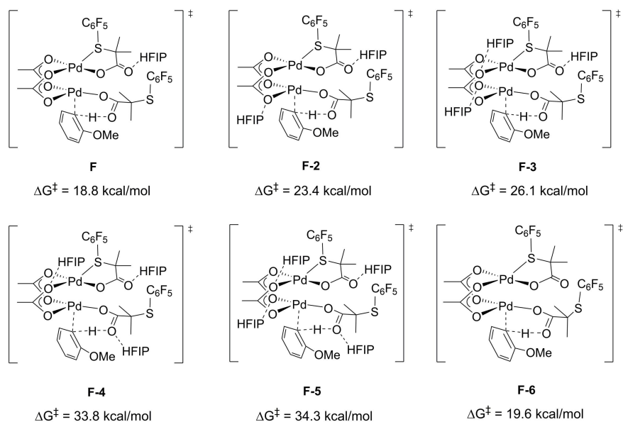
Fig. S2. The effect of noncovalent interactions between the HFIP molecules with both the substrate and the catalyst for Pd catalyzed C–H bond activation.
