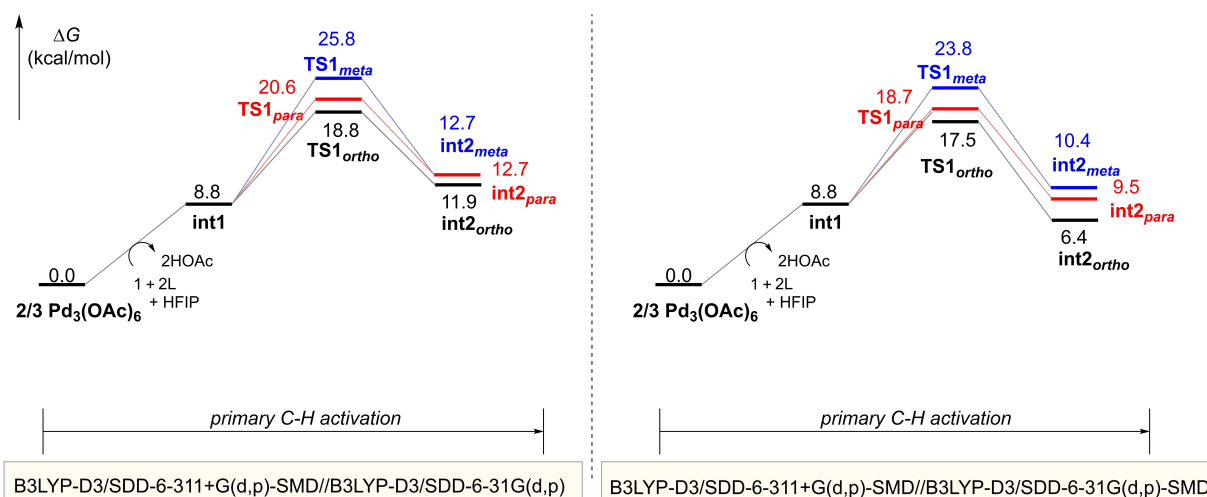
Fig. S3. Free energy profiles for C–H activation based on the structure optimized in the gas-phase and in HFIP solvent, the difference is small and consistent trends.
