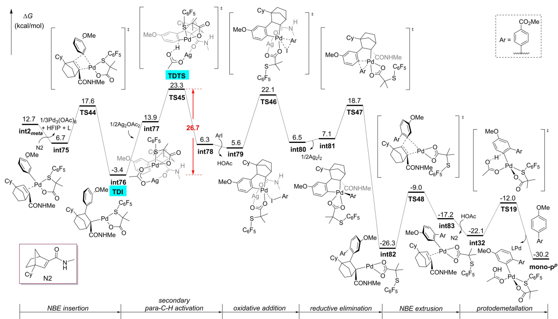
Fig. S12. Free energy profiles for the formation of mono-p''' from primary meta -C-H activation in the N2 system.
