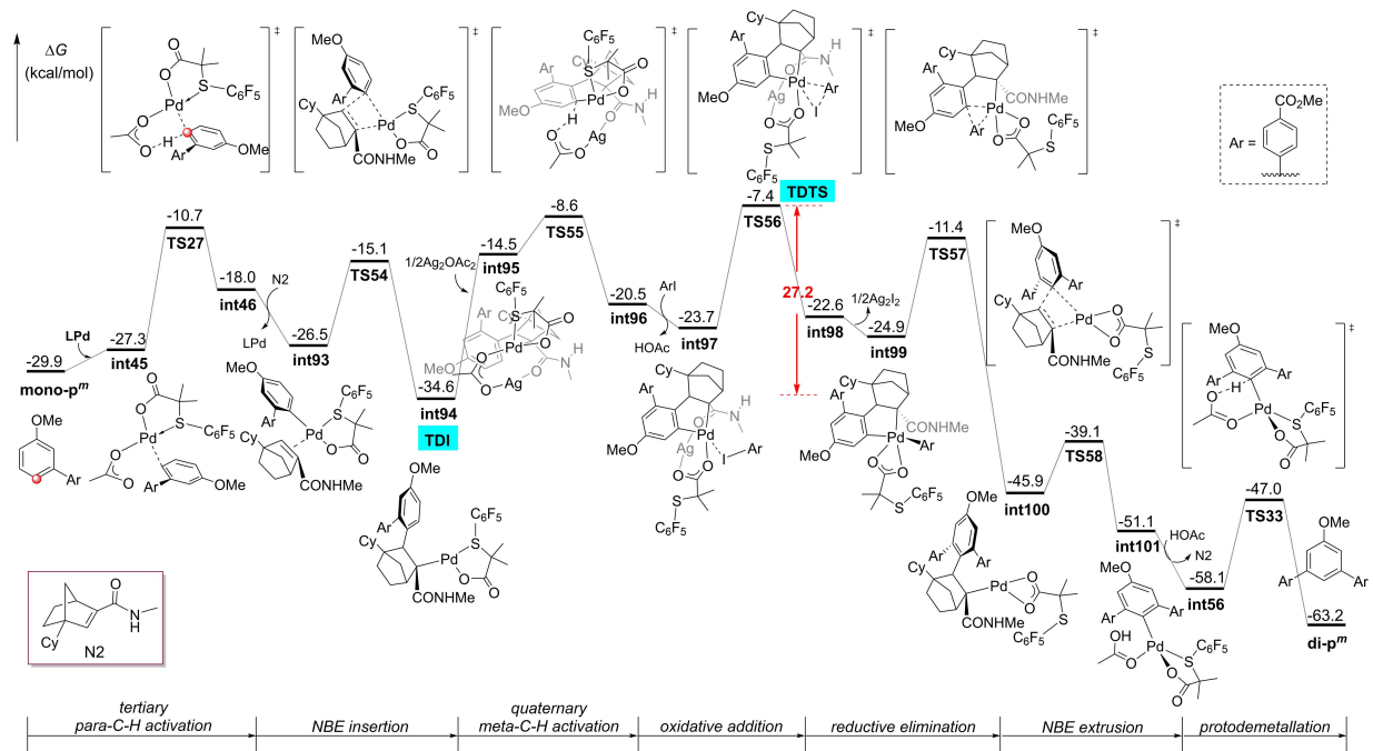
Fig. S14. Free energy profiles for the formation of di-p m from tertiary para -C-H activation in the N2 system.
