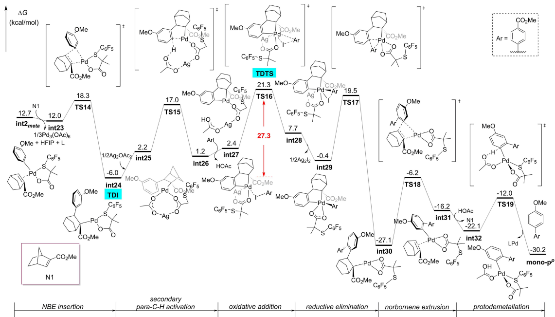
Fig. S7. Free energy profiles for the formation of mono-p'' from primary meta -C–H activation in the N1 system.
