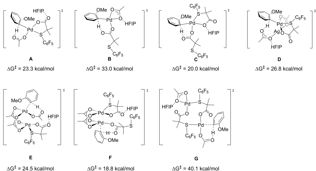
Fig. S1. Reaction free energies for the ortho -carbopalladation catalyzed by monomer or dimer palladium (the energies are respect to the \text{Pd}_3(\text{OAc})_6 trimer).
