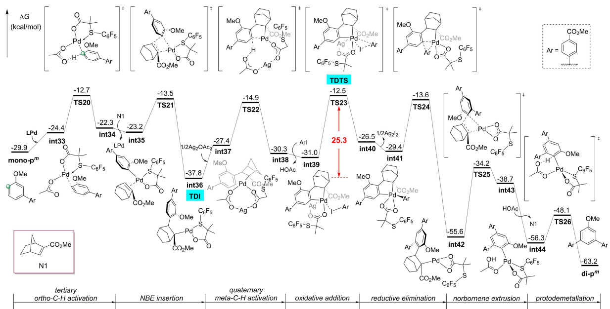
Fig. S8. Free energy profiles for the formation of di-p''' from tertiary ortho -C–H activation in the N1 system.
