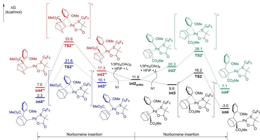
Fig. S5. Free energy profiles for four types of norbornene insertion.
