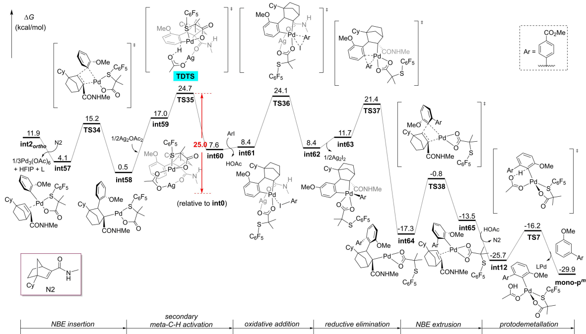
Fig. S10. Free energy profiles for the formation of mono-p m from primary ortho -C-H activation in the N2 system.
