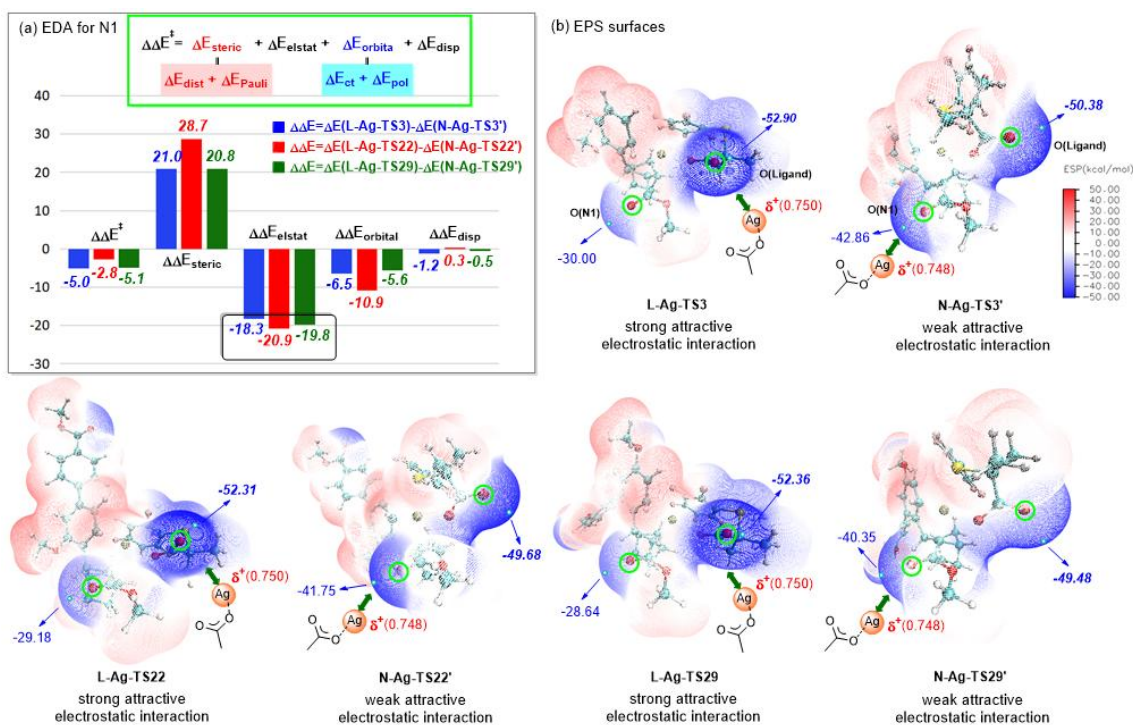
Fig. S15. Energy decomposition analysis in two conformations for secondary and quaternary meta -C–H activation in the N1 system.
