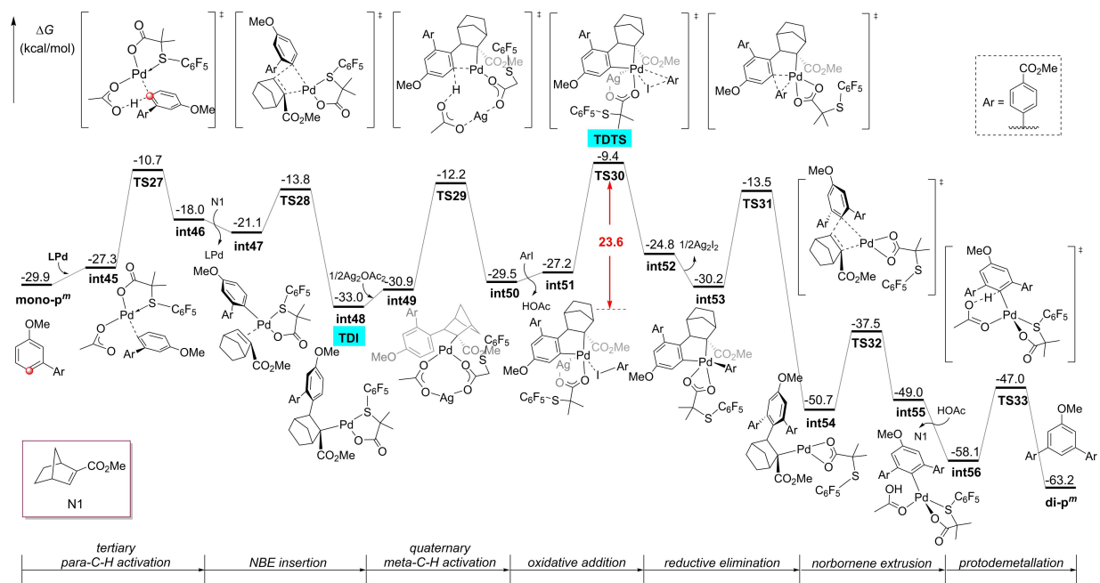
Fig. S9. Free energy profiles for the formation of di-p m from tertiary para -C-H activation in the N1 system.
