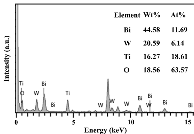
Fig. S1. EDS spectra of P25/BWO-20 heterojunction.
