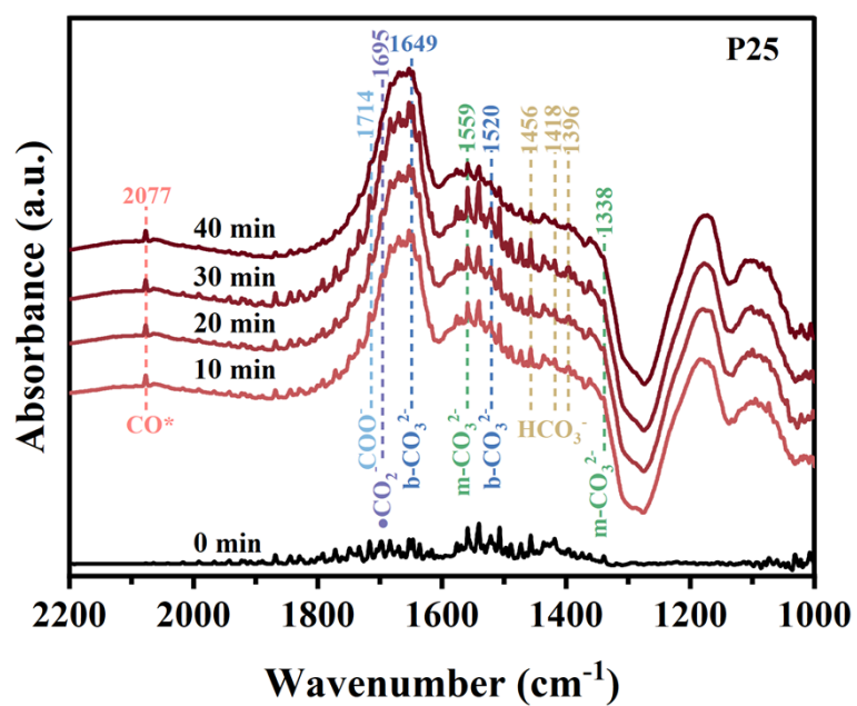
Fig. S4. In-situ DRIFTS spectra of surface adsorbed \text{CO}_2 species and photocatalytic \text{CO}_2 reduction intermediates of P25.
