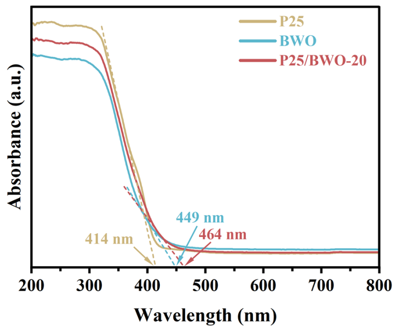
Fig. S3. UV-vis DRS of the as-prepared samples.
