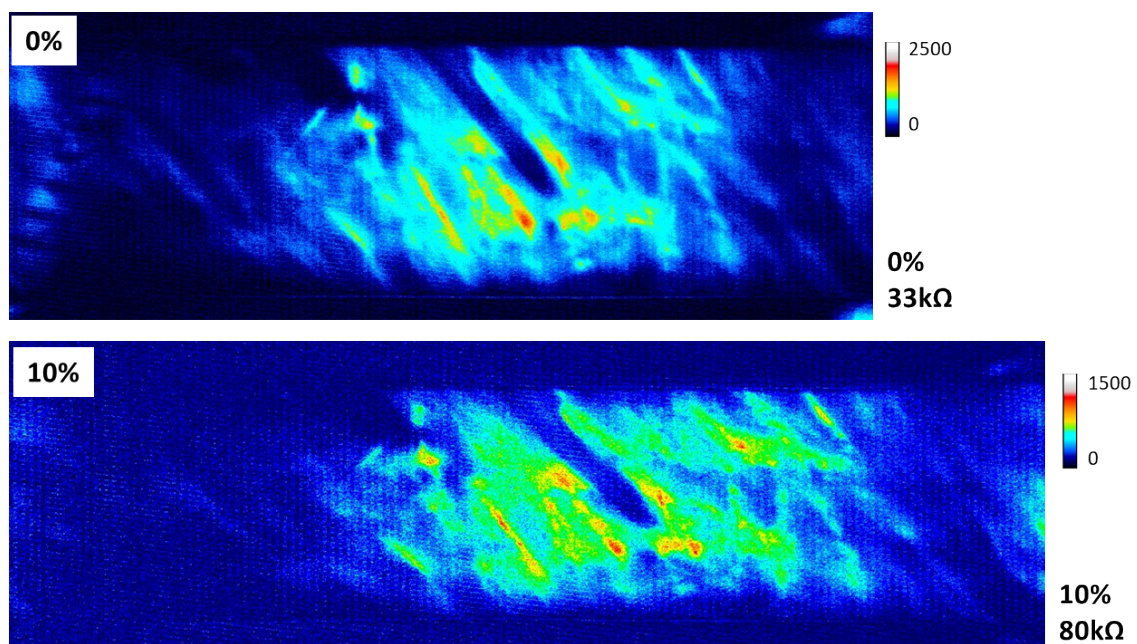
Fig. S1 LIT images of another CNT/FKM composite.
