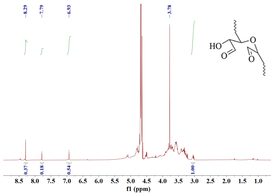
Figure S1. ^1\text{H} NMR spectra of PDA under alkaline condition (pH=13).
