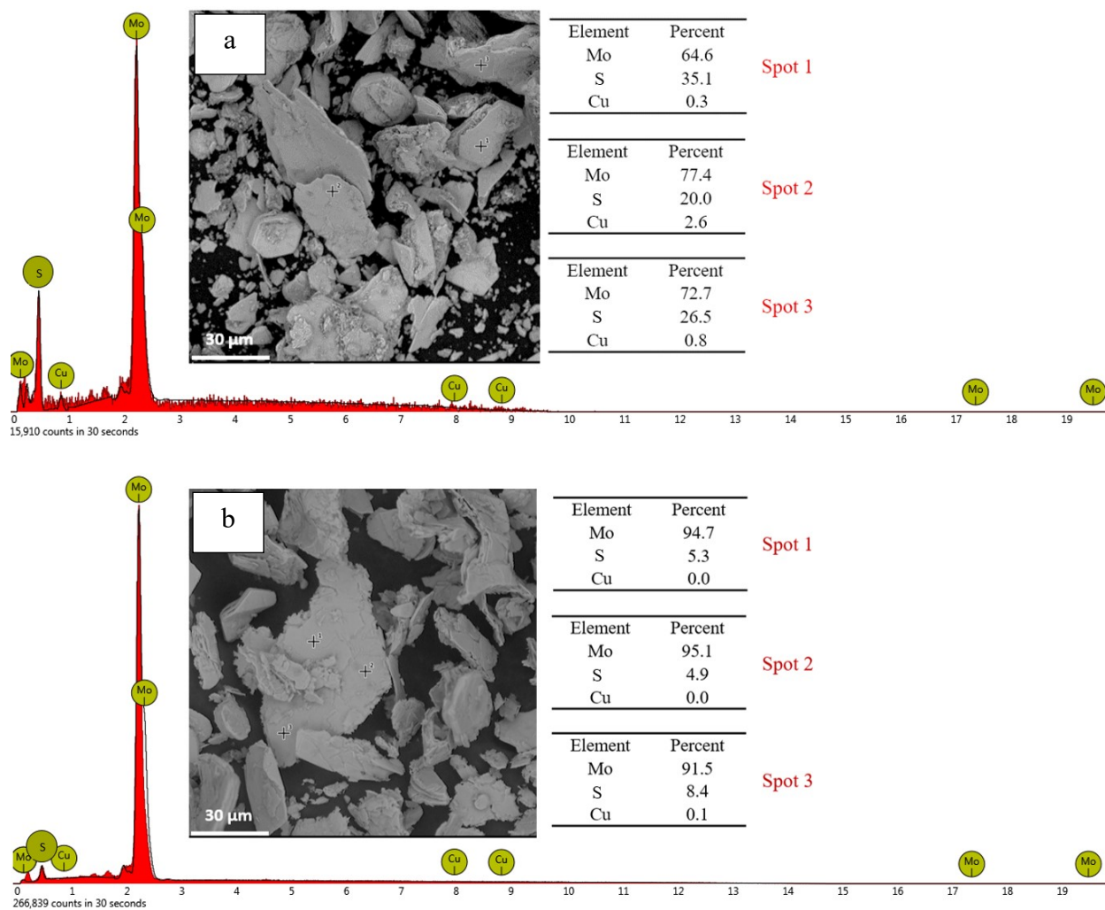
Figure S1. Figure 1. EDS analysis of (a) impure and (b) purified molybdenite concentrate.
