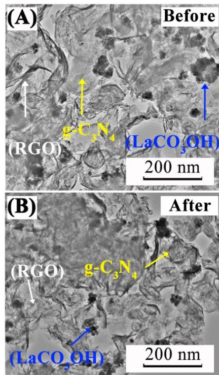
Figure S2. TEM images of RGO/g-C 3 N 4 /LaCO 3 OH before (A) and after (B) the cycling test.
