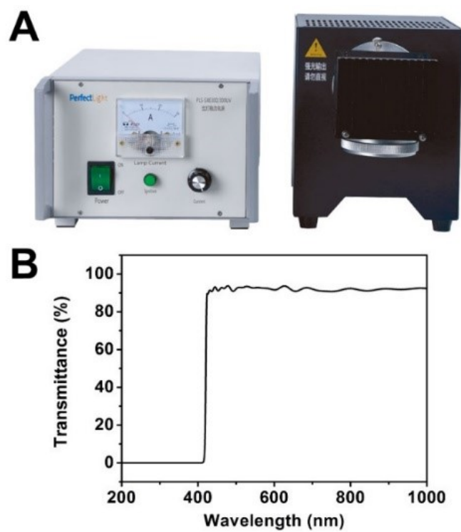
Figure S1. (A) The photograph of the 300 W xenon lamp (PLS-SXE 300, Beijing Perfect Light Co., Ltd.) and (B) the transmission spectrum of the filtered light.
