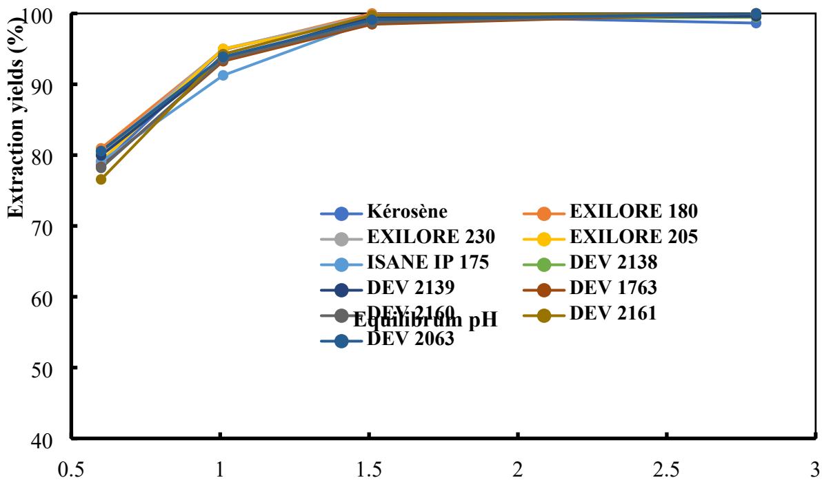
Figure S2: Extraction of copper by using Accorga M5640.
