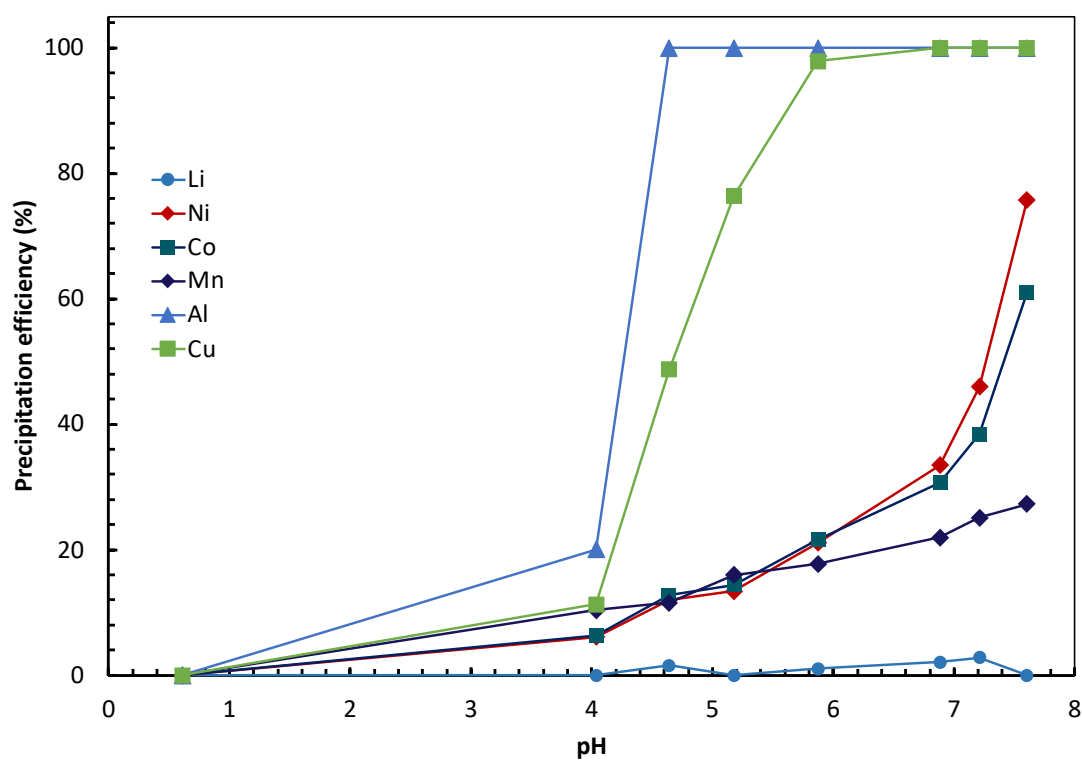
Figure S1: Precipitation curves as a function of pH.
