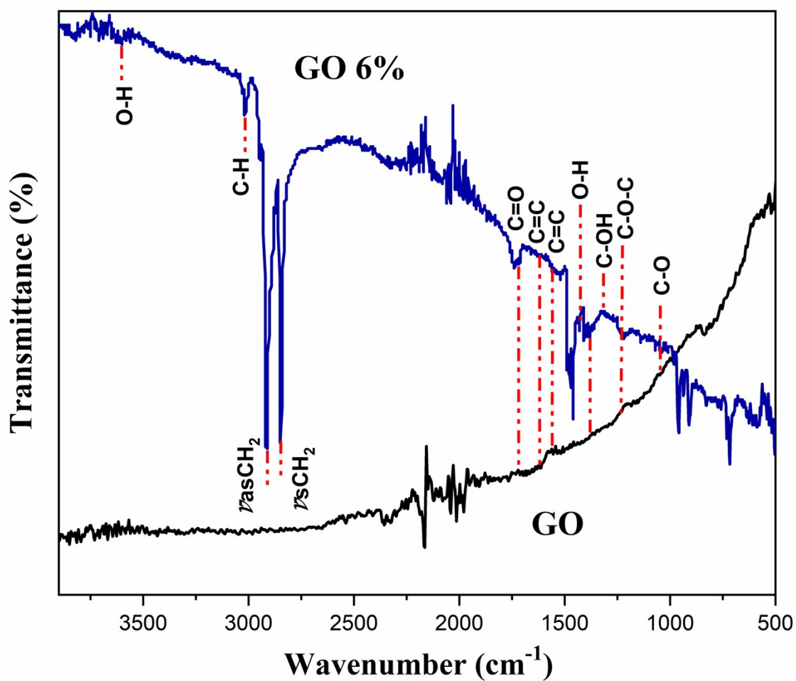
Figure S1. FTIR spectra of pure GO and GO 6%
