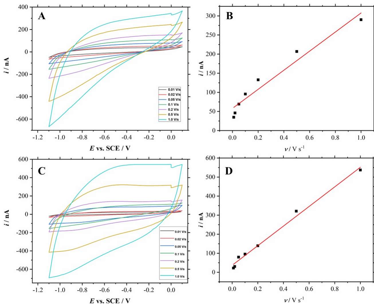
Figure S1: Cyclic voltammograms of smoothened (A) and roughened (C) Mo microdisk electrodes in N_2 -saturated 0.5 M KCl at different scan rates: 0.01, 0.02, 0.05, 0.1, 0.2, 0.5, and 1 V s^{-1} . Corresponding plots of current as a function of scan rate for the smoothened (B) and roughened (D) Mo microdisk electrodes. The currents were taken at around -0.2 V vs. SCE and the red lines resemble the fitting of the data.
