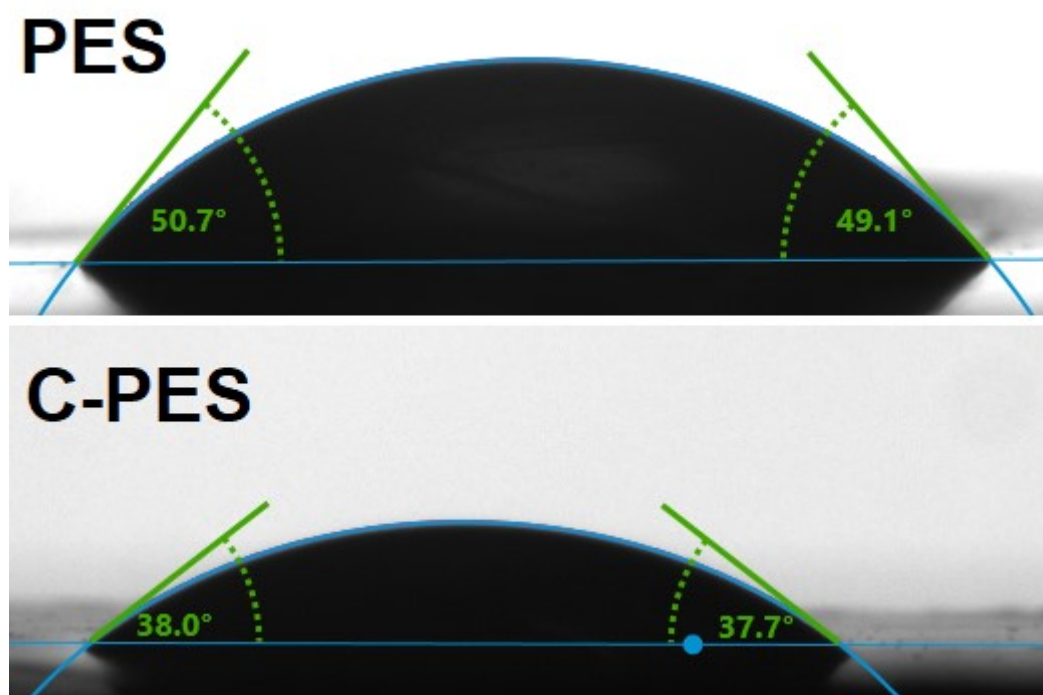
Figure 1s. Optical image of the water contact angle analysis of the reference PES and composite PES membranes.
