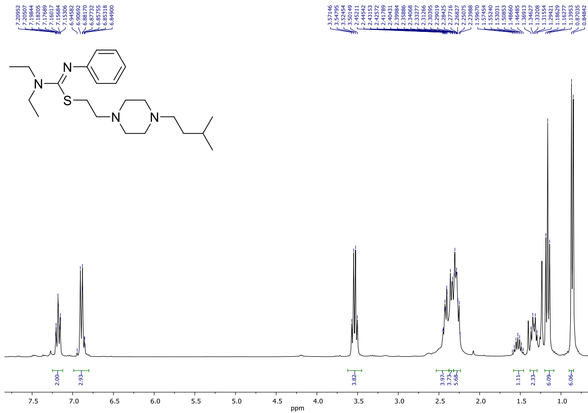
1 H NMR (300 MHz, CDCl 3 ); 2-(4-Isopentylpiperazin-1-yl) ethyl (Z)-N,N-diethyl-N'-phenylcarbamidithioate 3c
