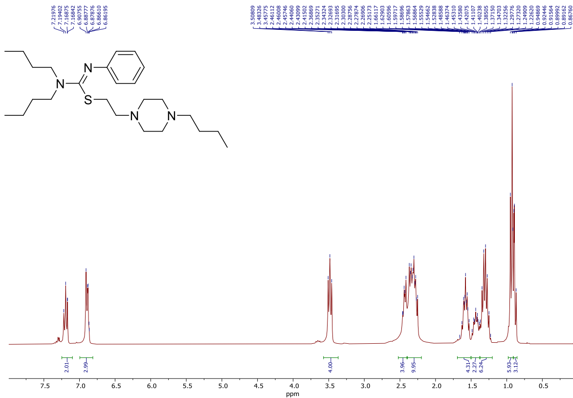
1 H NMR (75 MHz, CDCl 3 ); 2-(4-Butylpiperazin-1-yl)ethyl (Z)-N,N-dibutyl-N'-phenylcarbamimidothioate 3f
