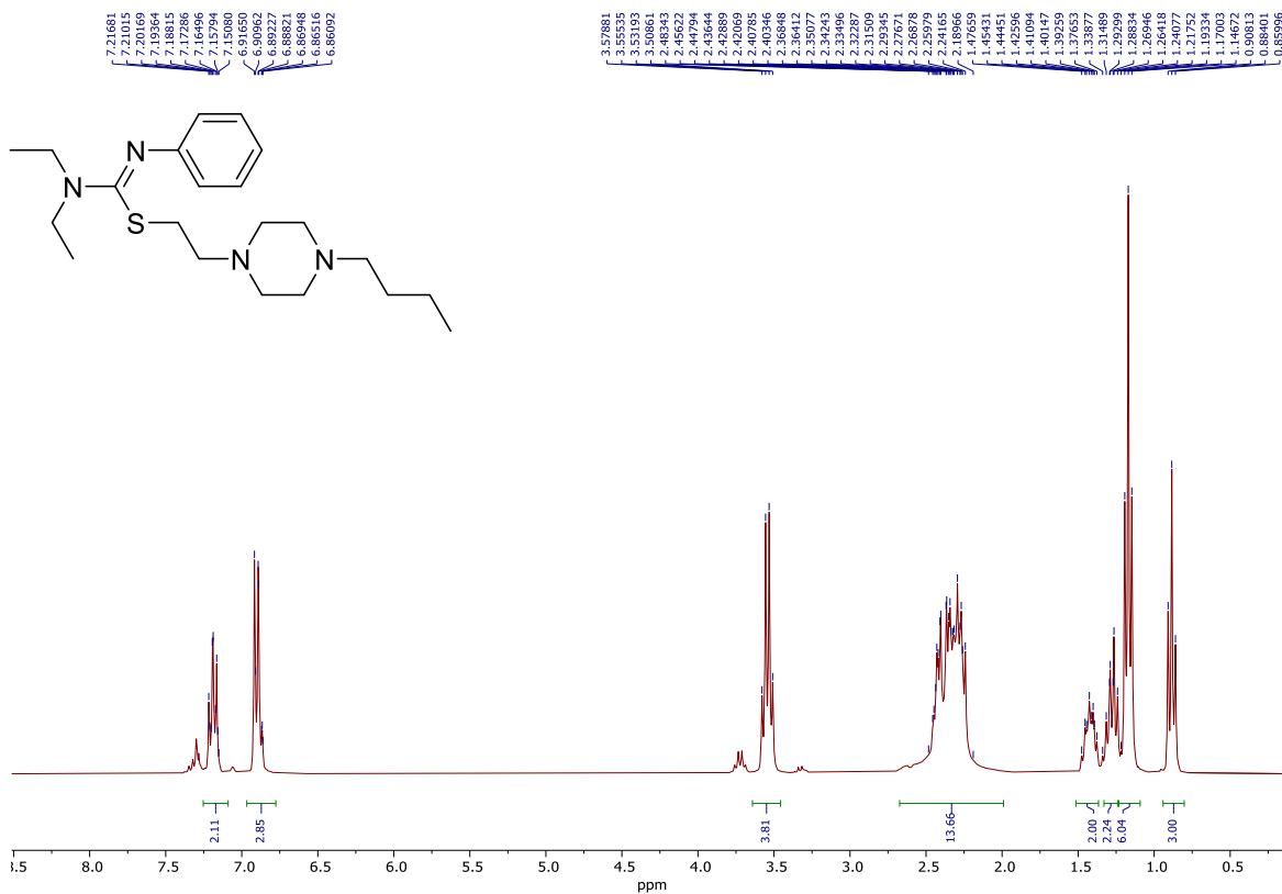
1 H NMR (300 MHz, CDCl 3 ); 2-(4-Butylpiperazin-1-yl) ethyl (Z)-N,N-diethyl-N'-phenylcarbamimidothioate 3d
