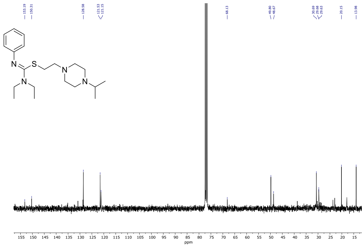
13 C NMR (75 MHz, CDCl 3 ); 2-(4-Isopropylpiperazin-1-yl)ethyl (Z)-N,N-diethyl-N'-phenylcarbamimidothioate 3b
