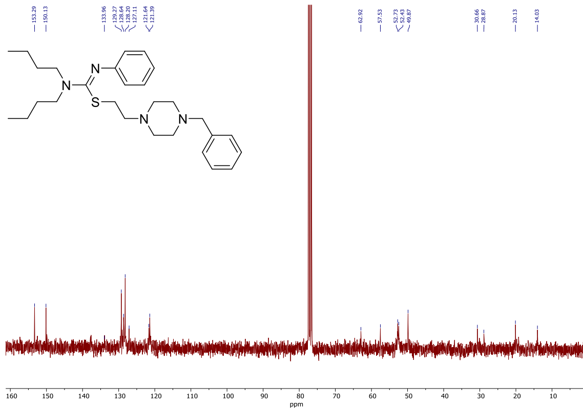
13 C NMR (75 MHz, CDCl 3 ); 2-(4-Benzylpiperazin-1-yl)ethyl (Z)-N,N-dibutyl-N'-phenylcarbamimidothioate 3g
