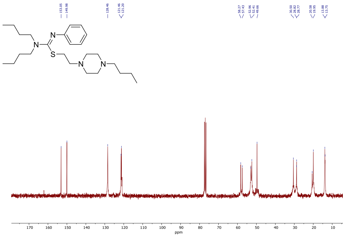
13 C NMR (75 MHz, CDCl 3 ); 2-(4-Butylpiperazin-1-yl)ethyl (Z)-N,N-dibutyl-N'-phenylcarbamimidothioate 3f
