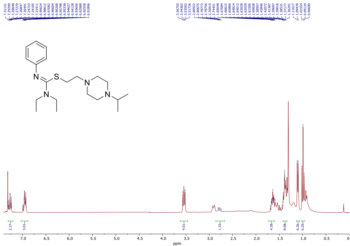
1 H NMR (300 MHz, CDCl 3 ); 2-(4-Isopropylpiperazin-1-yl)ethyl (Z)-N,N-diethyl-N'-phenylcarbamimidothioate 3b
