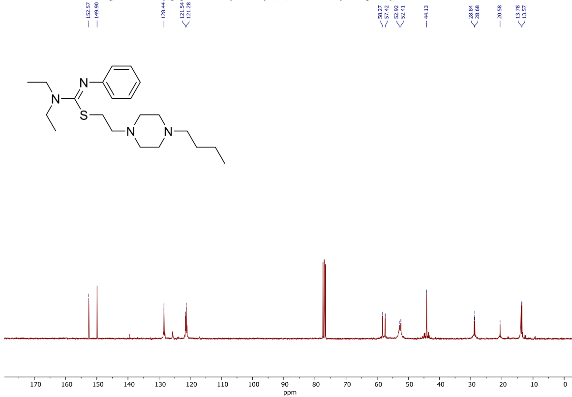
13 C NMR (75 MHz, CDCl 3 ); 2-(4-Butylpiperazin-1-yl) ethyl (Z)-N,N-diethyl-N'-phenylcarbamimidothioate 3d
