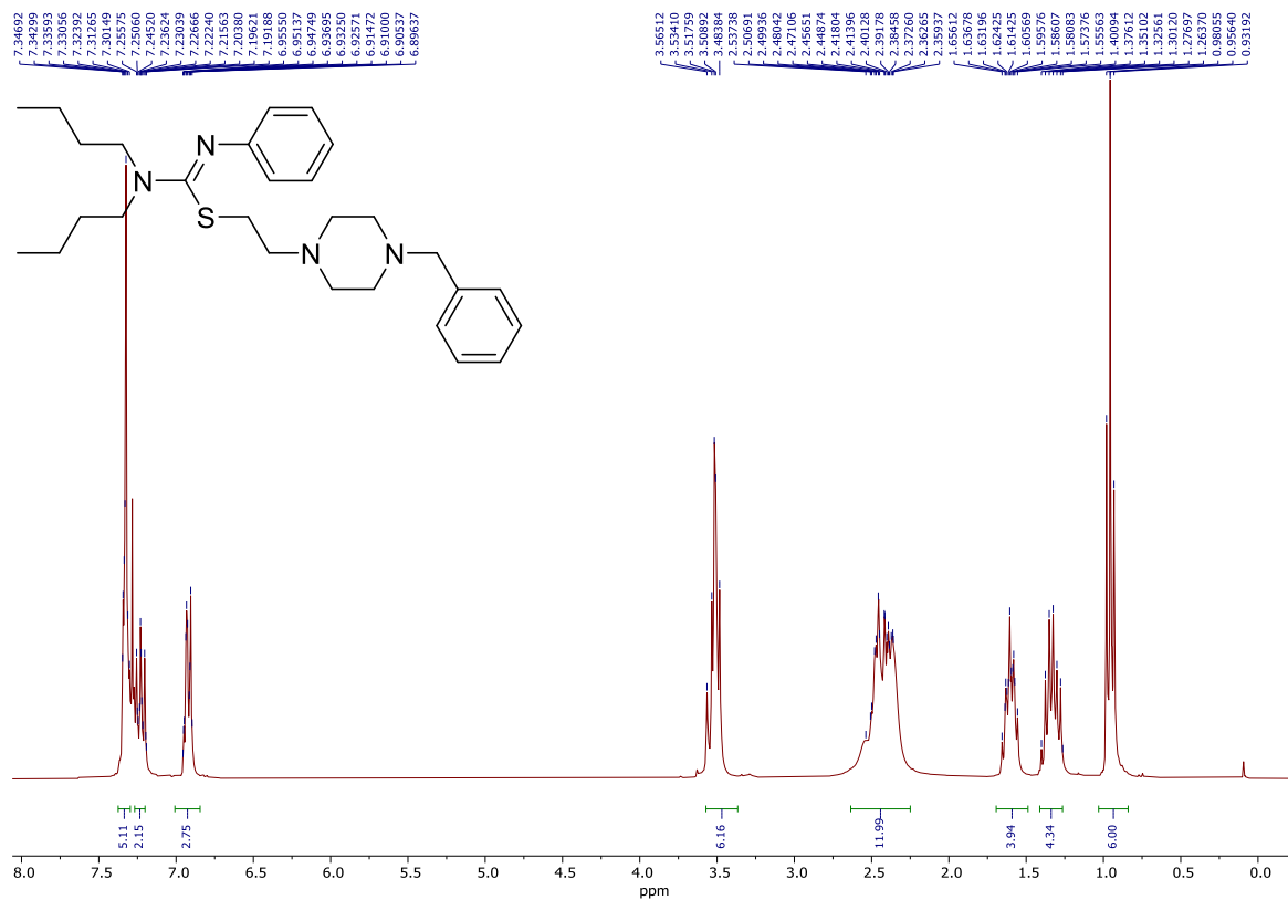
1 H NMR (300 MHz, CDCl 3 ); 2-(4-Benzylpiperazin-1-yl)ethyl (Z)-N,N-dibutyl-N'-phenylcarbamimidothioate 3g
