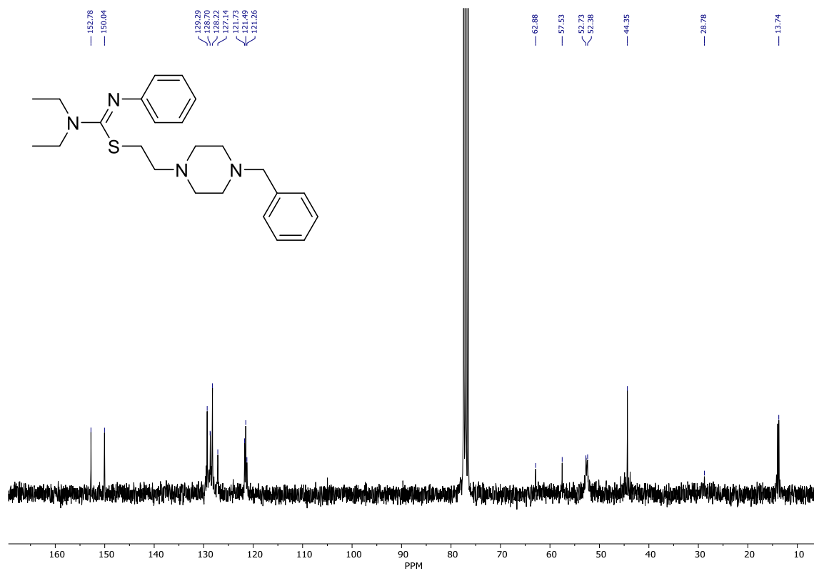
13 C NMR (75 MHz, CDCl 3 ); 2-(4-Benzylpiperazin-1-yl) ethyl (Z)-N,N-diethyl-N'-phenylcarbamimidothioate 3e
