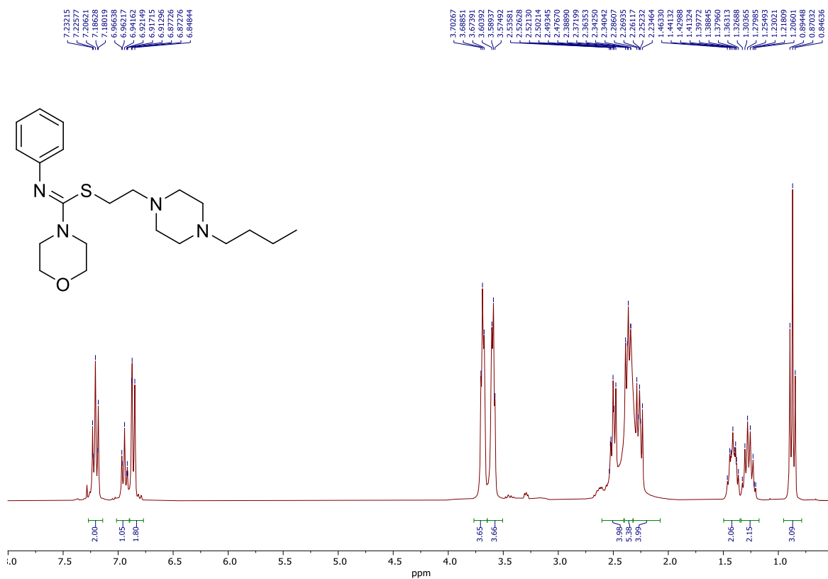
1 H NMR (300 MHz, CDCl 3 ); 2-(4-Butylpiperazin-1-yl)ethyl (Z)-N-phenylmorpholine-4-carbimidothioate 3h
