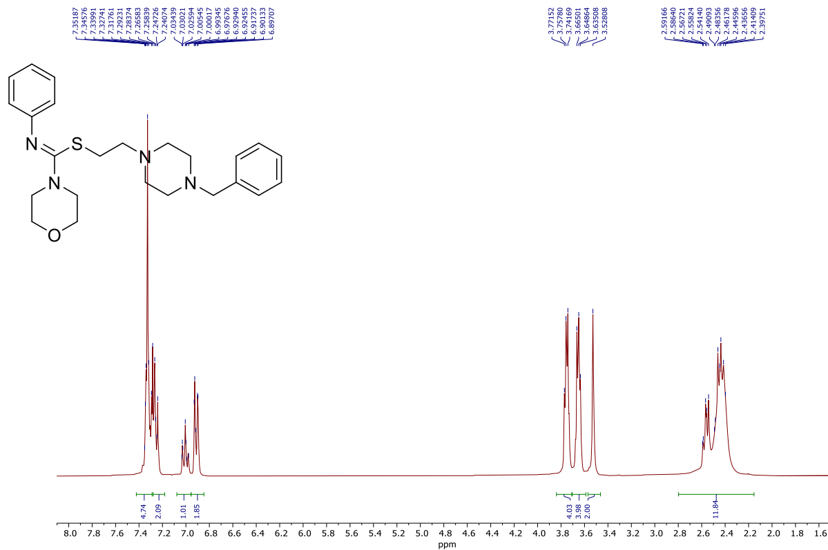
1 H NMR (75 MHz, CDCl 3 ); 2-(4-Benzylpiperazin-1-yl)ethyl (Z)-N-phenylmorpholine-4-carbimidothioate 3j
