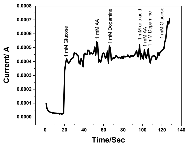
Figure S1: Chronoamperometry experiments conducted for glucose sensing in the presence of interferants.
