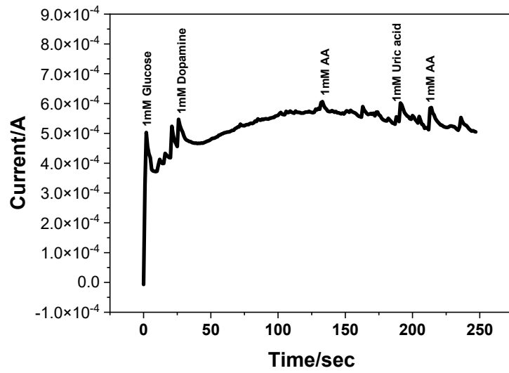
Figure S2: Chronoamperometry experiments conducted for glucose sensing in the presence of interferants.
