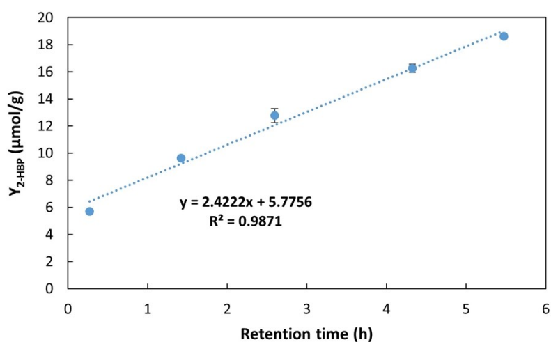
Fig. S2. Correlation between Y_{2-HBP} and retention time, when different volumes were tested on the BDS continuous system, with 35% n-heptane containing 500 \mu\text{M} of DBT (3.5:6.5 ratio).
