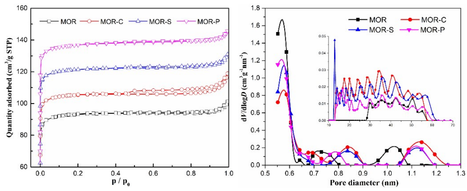
Fig. S1 N 2 adsorption and desorption isotherms (a) and pore size distribution (b) of MOR samples
