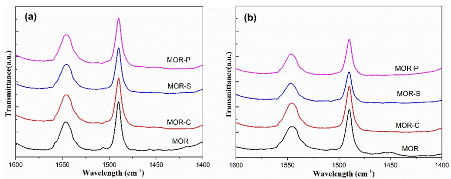
Fig. S2 Py-IR spectra of MOR synthesized with different soft template (a: Py desorpted at 150 °C; b: Py desorpted at 300 °C)
