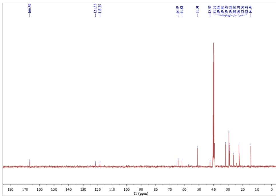
Fig. S2 ^{13}\text{C} NMR spectrum of [Laur][Tf 2 N].
