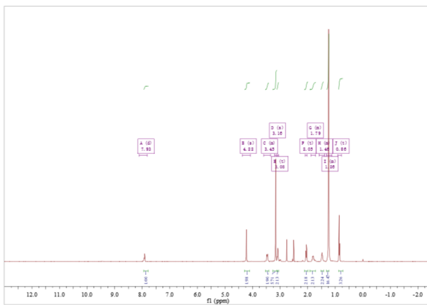
Fig. S3 ^1\text{H} NMR spectrum of [Coca][Tf 2 N].
