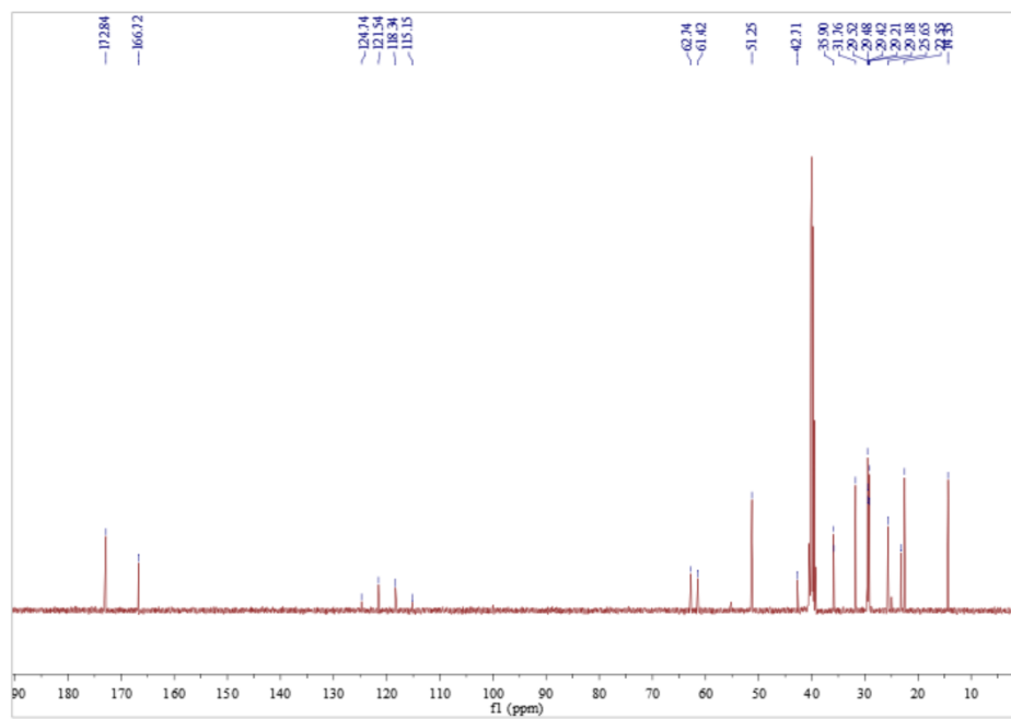
Fig. S4 ^{13}\text{C} NMR spectrum of [Coca][Tf 2 N].
