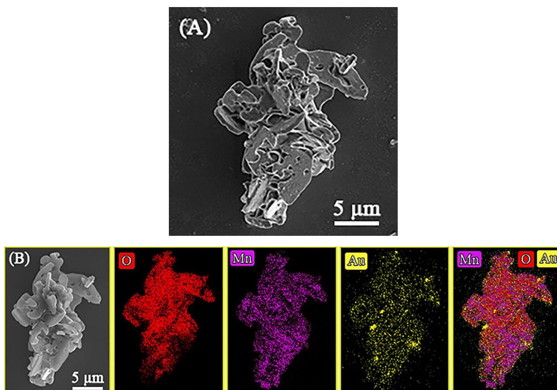
Fig. S2 (A) SEM images, (B) element distribution of O, Mn and Au species over SEM-EDX of Au-Mn 3 O 4 .
