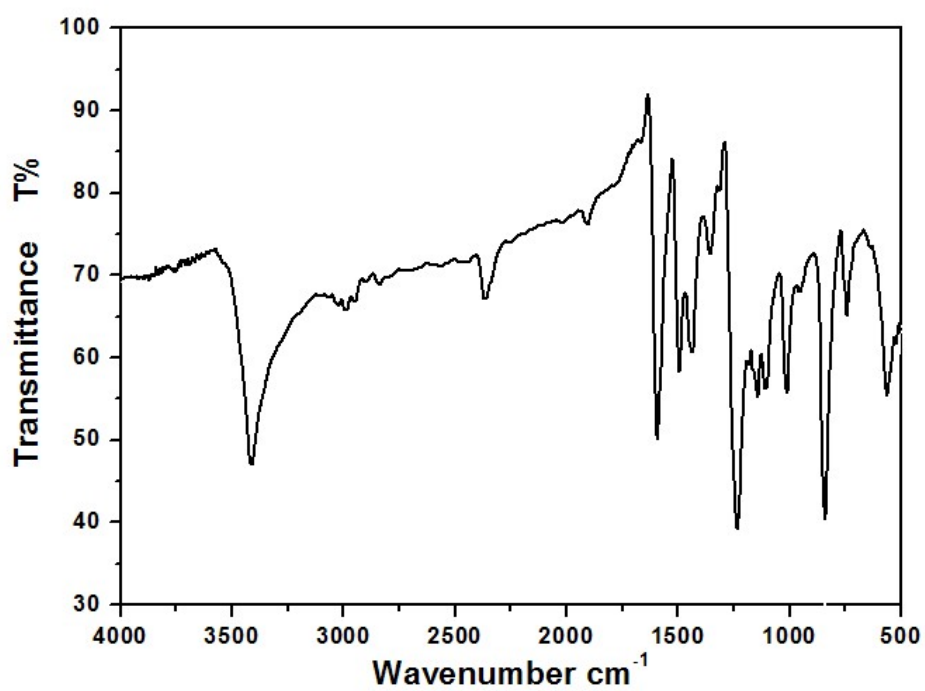
Fig. S3. FT-IR spectrum of Azo2.
