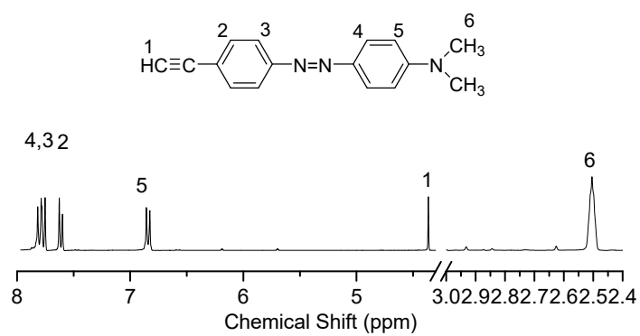
Fig. S5. 1 H NMR of Azo1.
