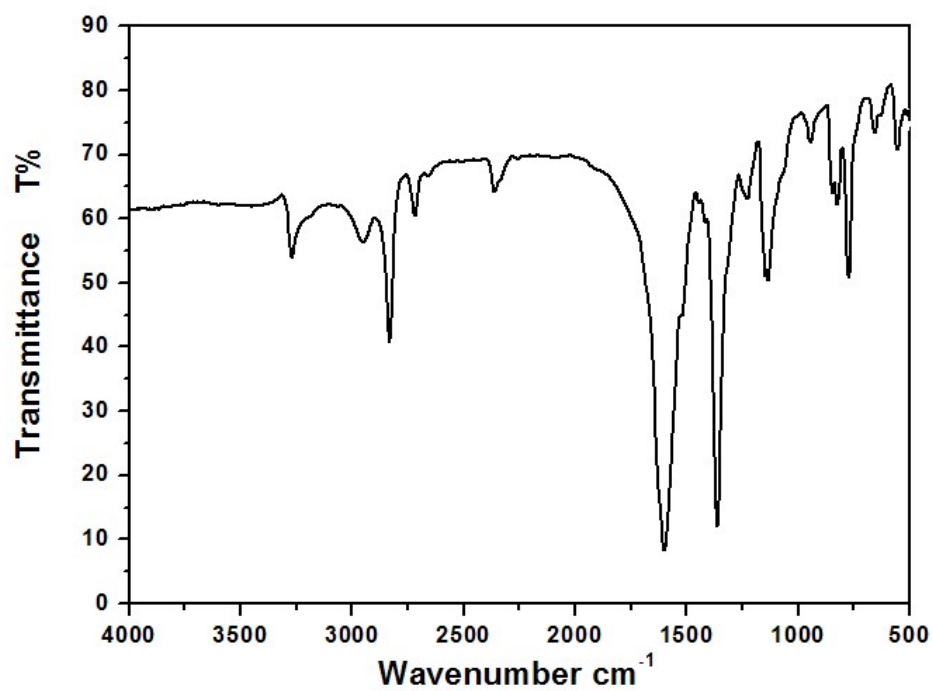
Fig. S2. FT-IR spectrum of Azo1
