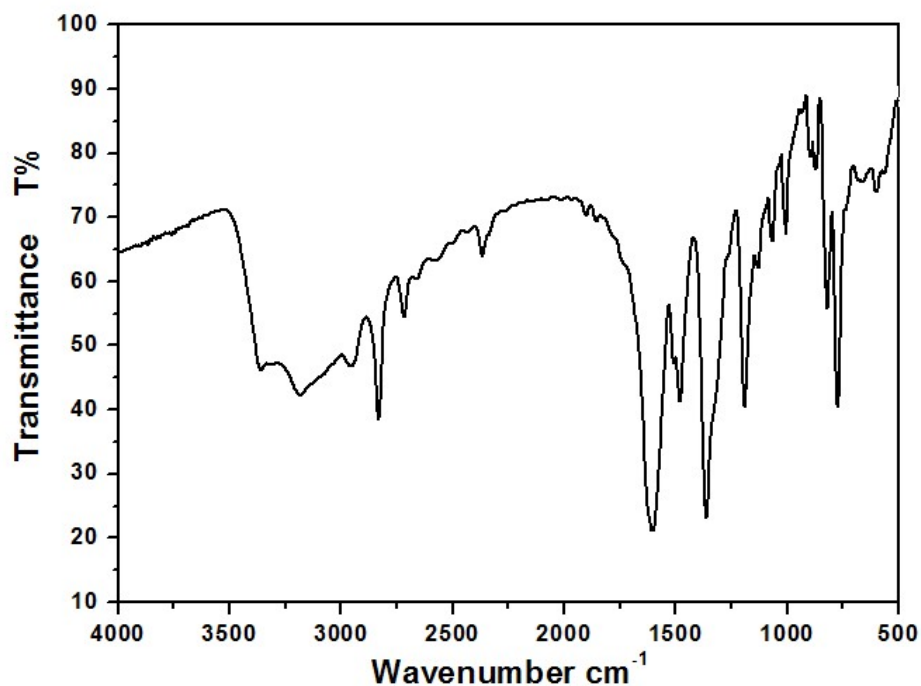
Fig. S1. FT-IR spectrum of 2- (4 ' - bromophenyl) hydroquinone
