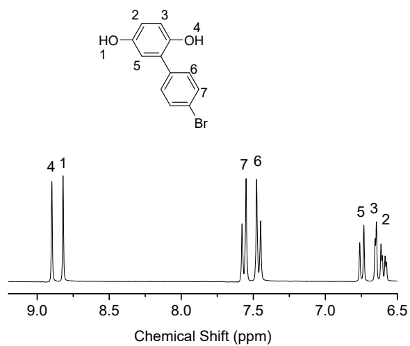
Fig. S4. 1 H NMR of 2- (4'- bromophenyl) hydroquinone.
