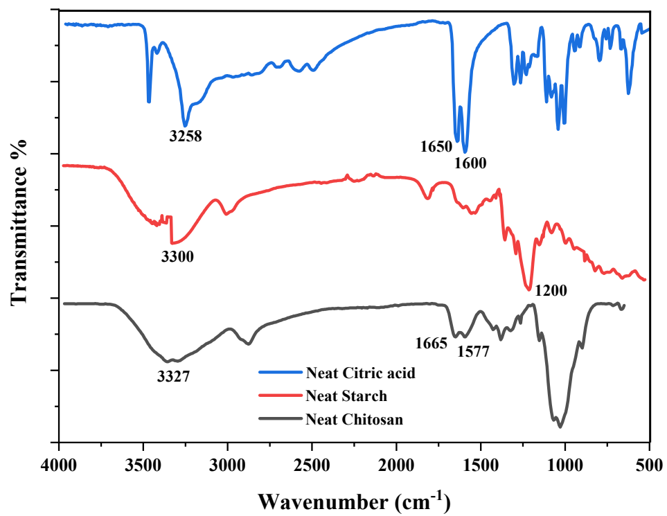
Fig S1. FTIR spectra of neat components
