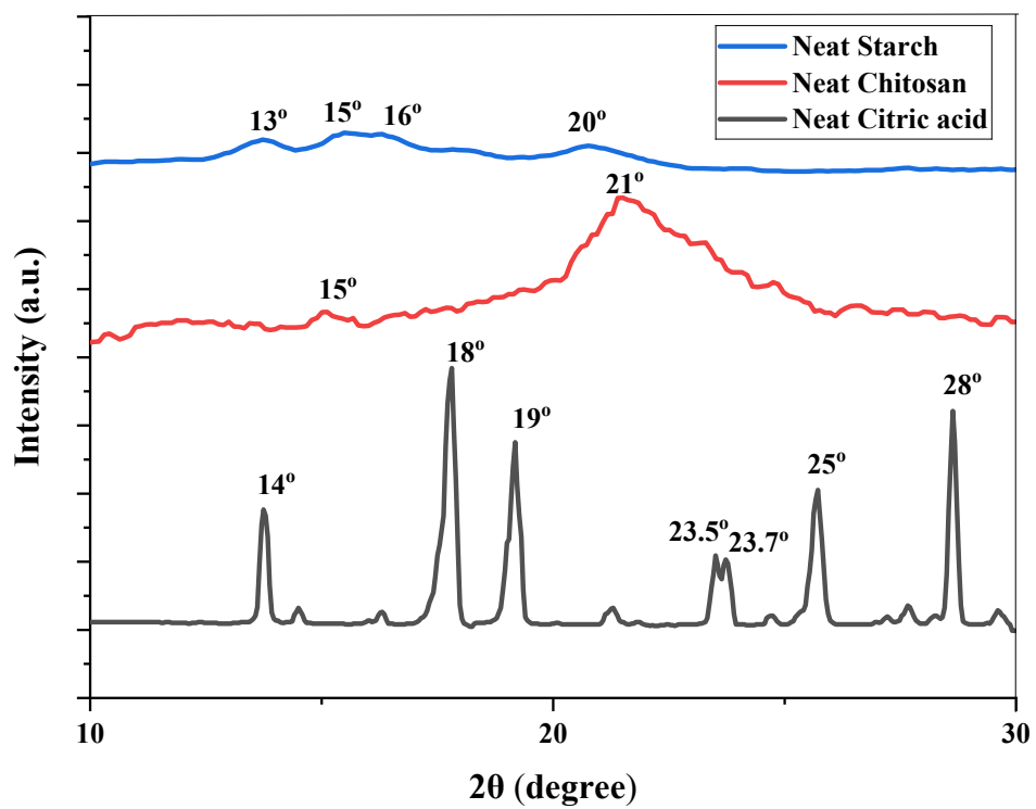
Fig. S2 XRD graphs of neat components
