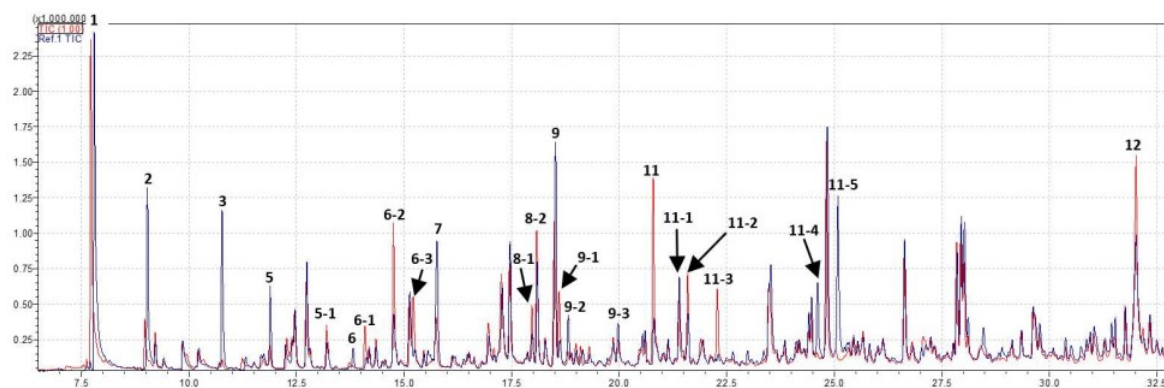
Figure S1. Sargassum oil chromatogram: SG Char (blue) superposed on Sargassum oil SIC (red) - (Zoom 6-33 minutes).
