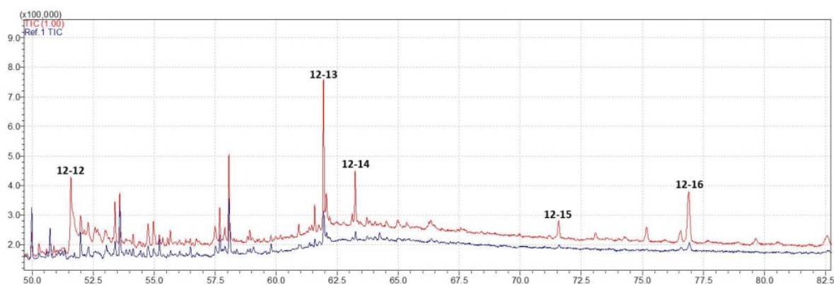
Figure S3. Sargassum oil chromatogram: SG Char (blue) superposed on Sargassum oil SIC (red) - (Zoom 50 – 82.5 minutes).
