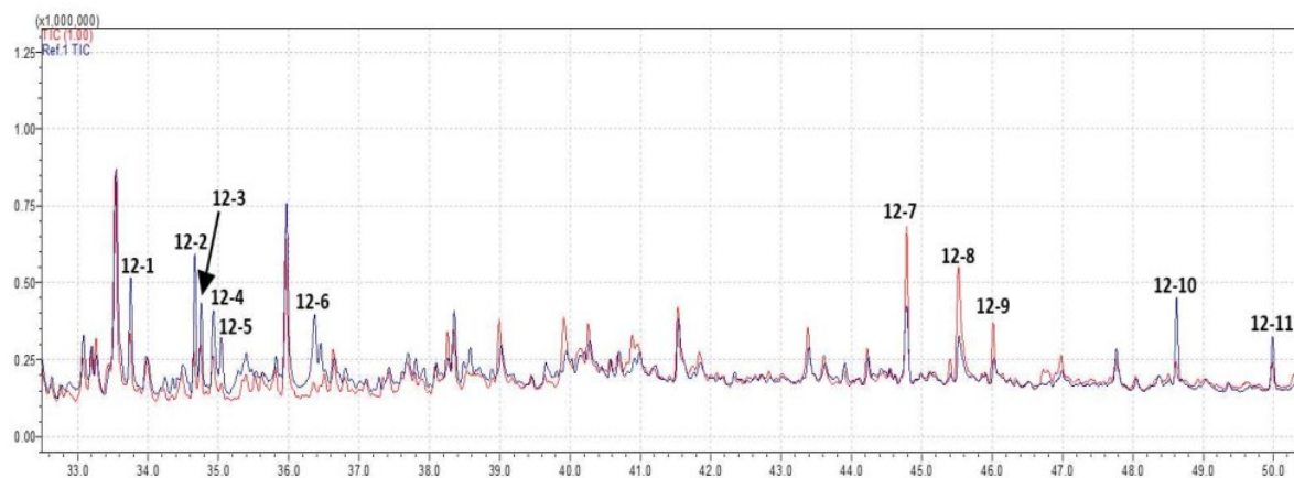
Figure S2. Sargassum oil chromatogram: SG Char (blue) superposed on Sargassum oil SIC (red) - (Zoom 33 - 50 minutes).
