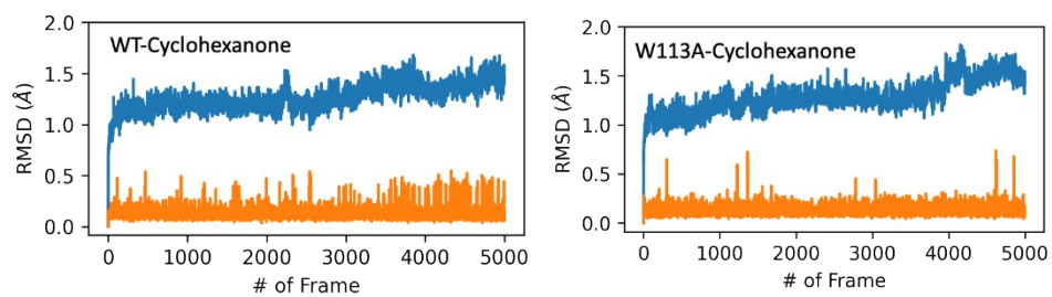
Figure S10. The RMSD obtained from wild type CDH and W113A in complex with cyclohexanone ligand for 500 ns trajectory. The RMSD values of C \alpha atoms of the protein and the heavy atoms of cyclohexanone ligand are shown in blue and orange colours respectively.
