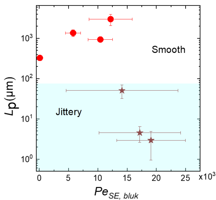
FIG. 1: Variation of persistence length ( L_p ) with Péclet number ( Pe_{SE, bulk} ) obtained using micelle diffusivity calculated via the Stokes-Einstein relationship with bulk phase viscosity ( \eta_b ).
