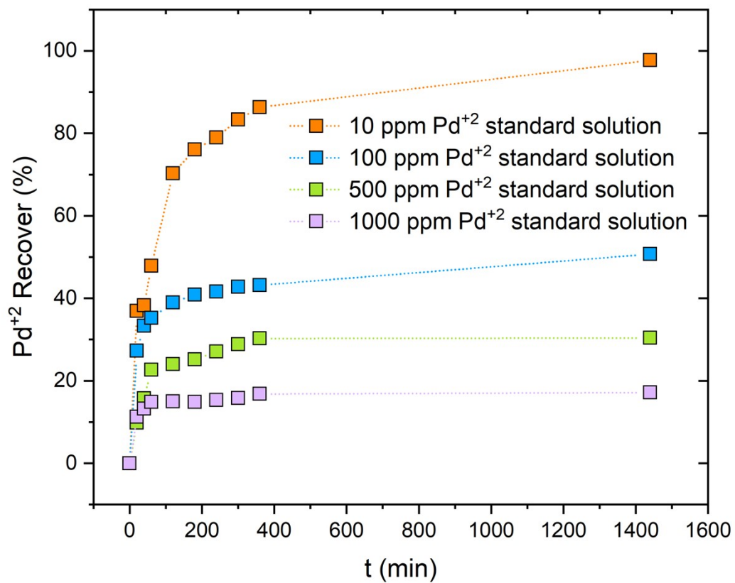
Figure 2S. Palladium recovery % according to batch adsorption for different initial Palladium feed solutions.
